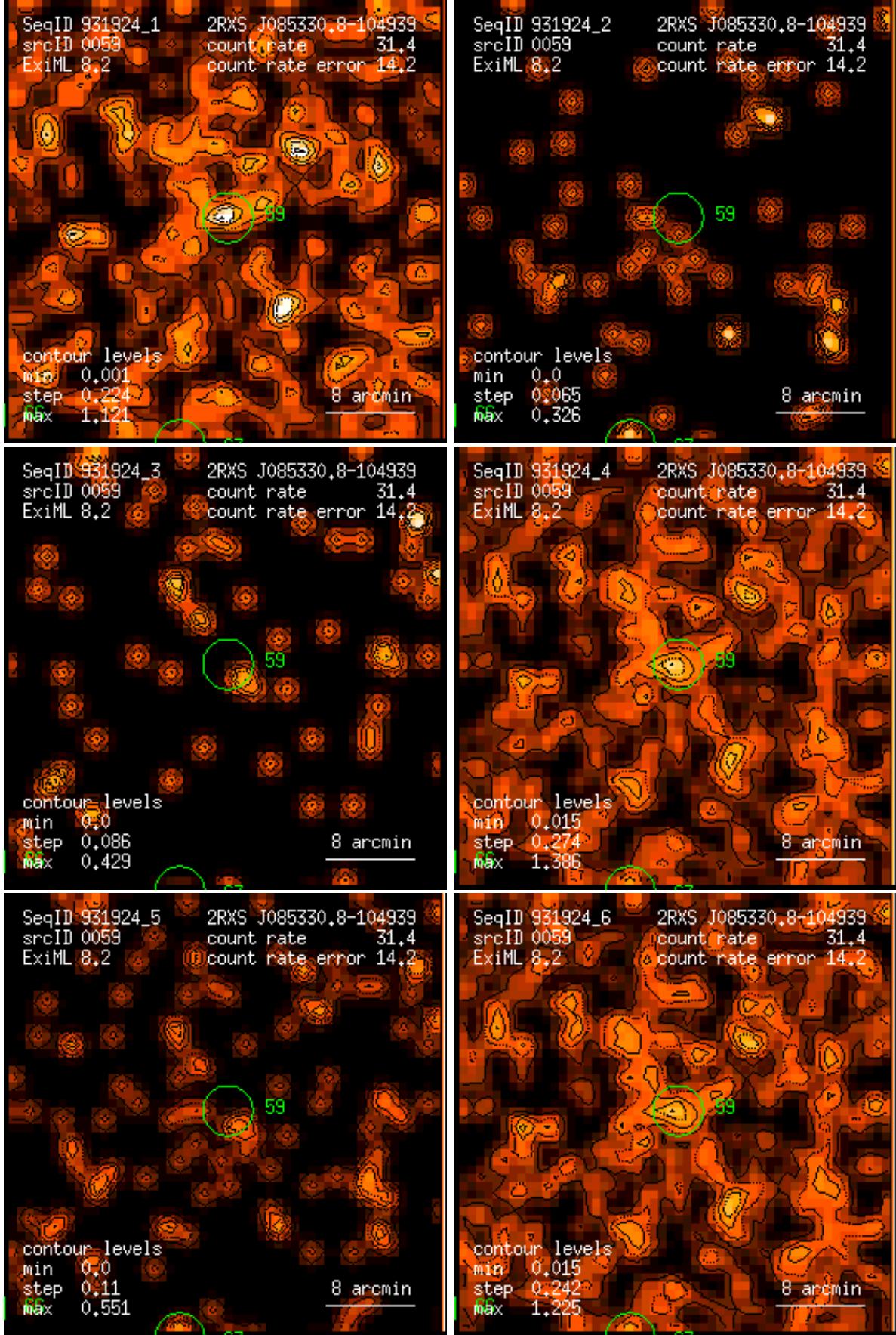
Figure 59: RASS 931924: detection 0059: band rate images, Gaussian filter: (1) PSPC channels 11 – 41, (2) 52 – 90, (3) 91 – 201, (4) 11 – 235, (5) 52 – 201, (6) 11 – 201. Broad band rates in counts/ks. Band rate contour levels in counts/ks/arcmin 2 .
