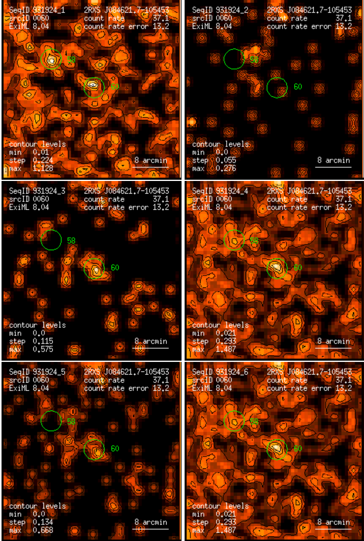
Figure 60: RASS 931924: detection 0060: band rate images, Gaussian filter: (1) PSPC channels 11 – 41, (2) 52 – 90, (3) 91 – 201, (4) 11 – 235, (5) 52 – 201, (6) 11 – 201. Broad band rates in counts/ks. Band rate contour levels in counts/ks/arcmin 2 .
