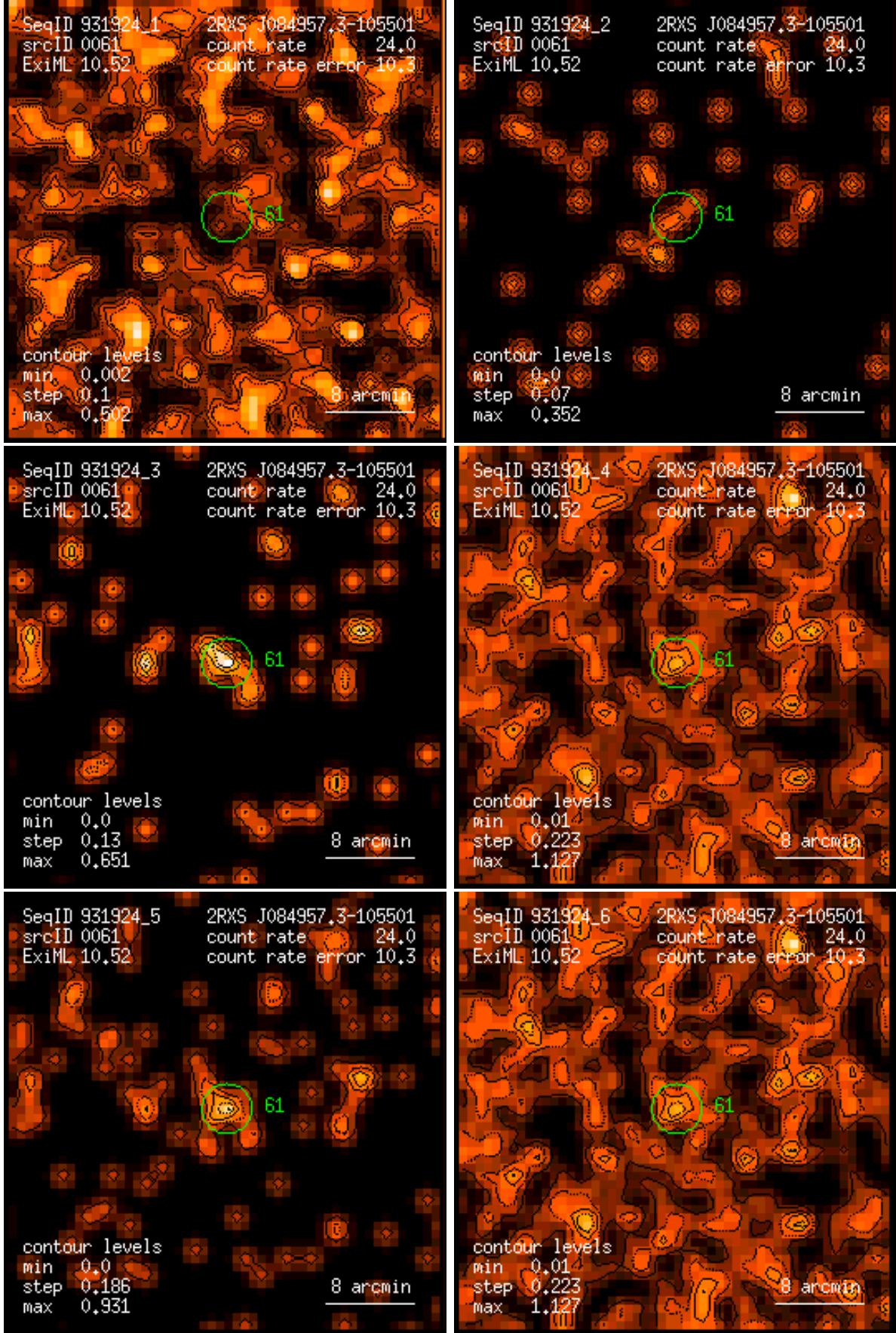
Figure 61: RASS 931924: detection 0061: band rate images, Gaussian filter: (1) PSPC channels 11 – 41, (2) 52 – 90, (3) 91 – 201, (4) 11 – 235, (5) 52 – 201, (6) 11 – 201. Broad band rates in counts/ks. Band rate contour levels in counts/ks/arcmin 2 .
