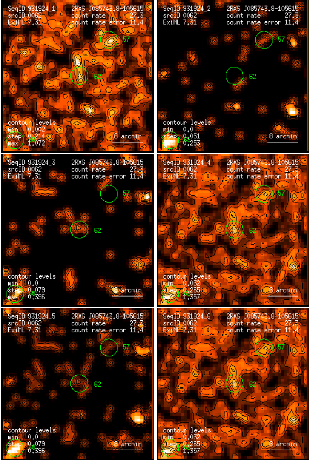
Figure 62: RASS 931924: detection 0062: band rate images, Gaussian filter: (1) PSPC channels 11 – 41, (2) 52 – 90, (3) 91 – 201, (4) 11 – 235, (5) 52 – 201, (6) 11 – 201. Broad band rates in counts/ks. Band rate contour levels in counts/ks/arcmin 2 .
