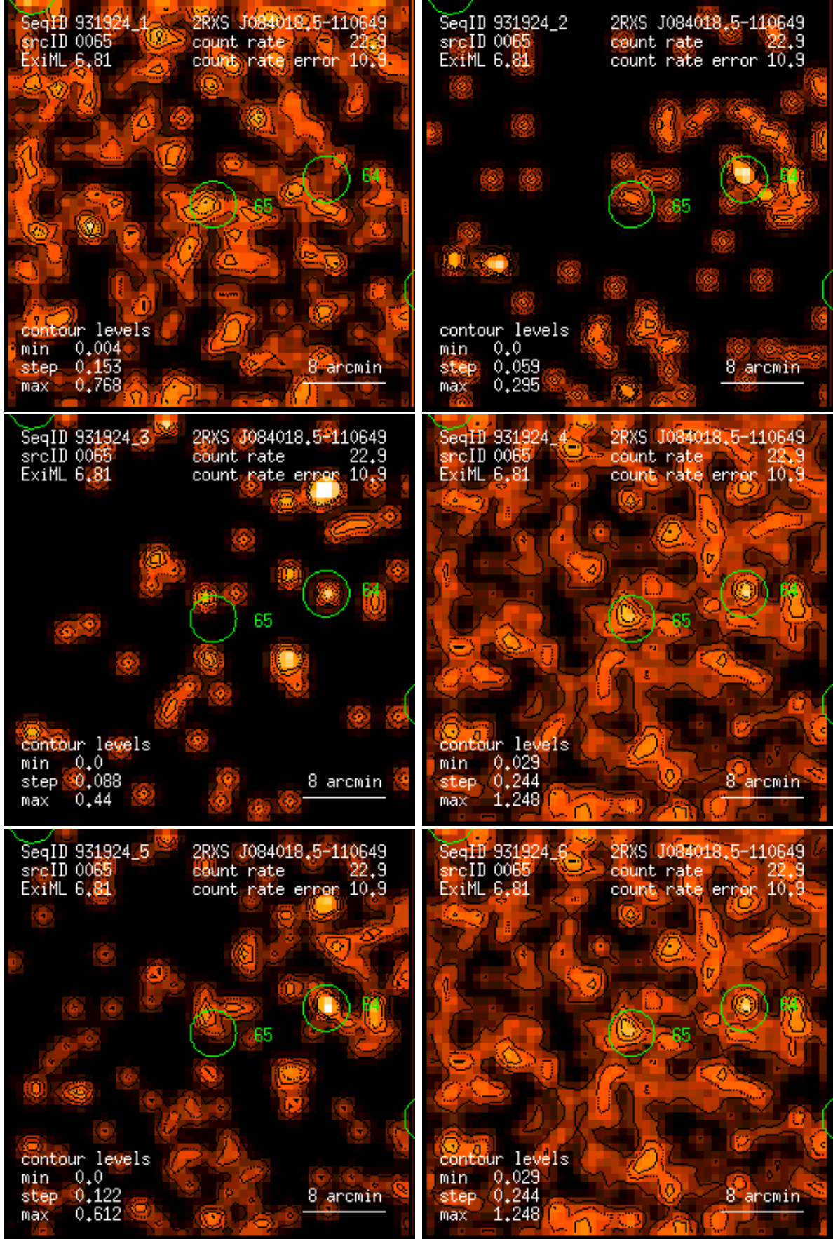
Figure 65: RASS 931924: detection 0065: band rate images, Gaussian filter: (1) PSPC channels 11 – 41, (2) 52 – 90, (3) 91 – 201, (4) 11 – 235, (5) 52 – 201, (6) 11 – 201. Broad band rates in counts/ks. Band rate contour levels in counts/ks/arcmin 2 .
