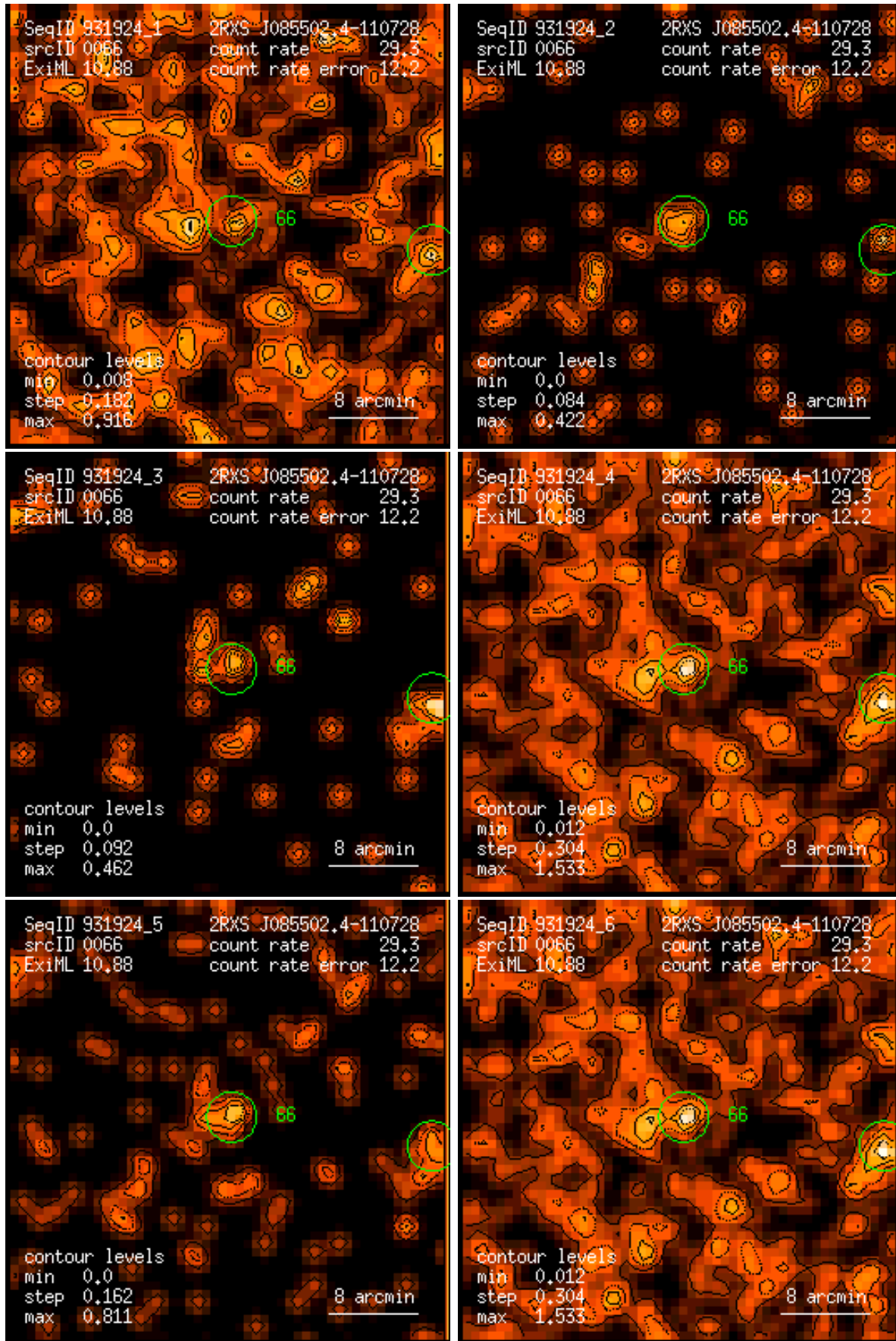
Figure 66: RASS 931924: detection 0066: band rate images, Gaussian filter: (1) PSPC channels 11 – 41, (2) 52 – 90, (3) 91 – 201, (4) 11 – 235, (5) 52 – 201, (6) 11 – 201. Broad band rates in counts/ks. Band rate contour levels in counts/ks/arcmin 2 .
