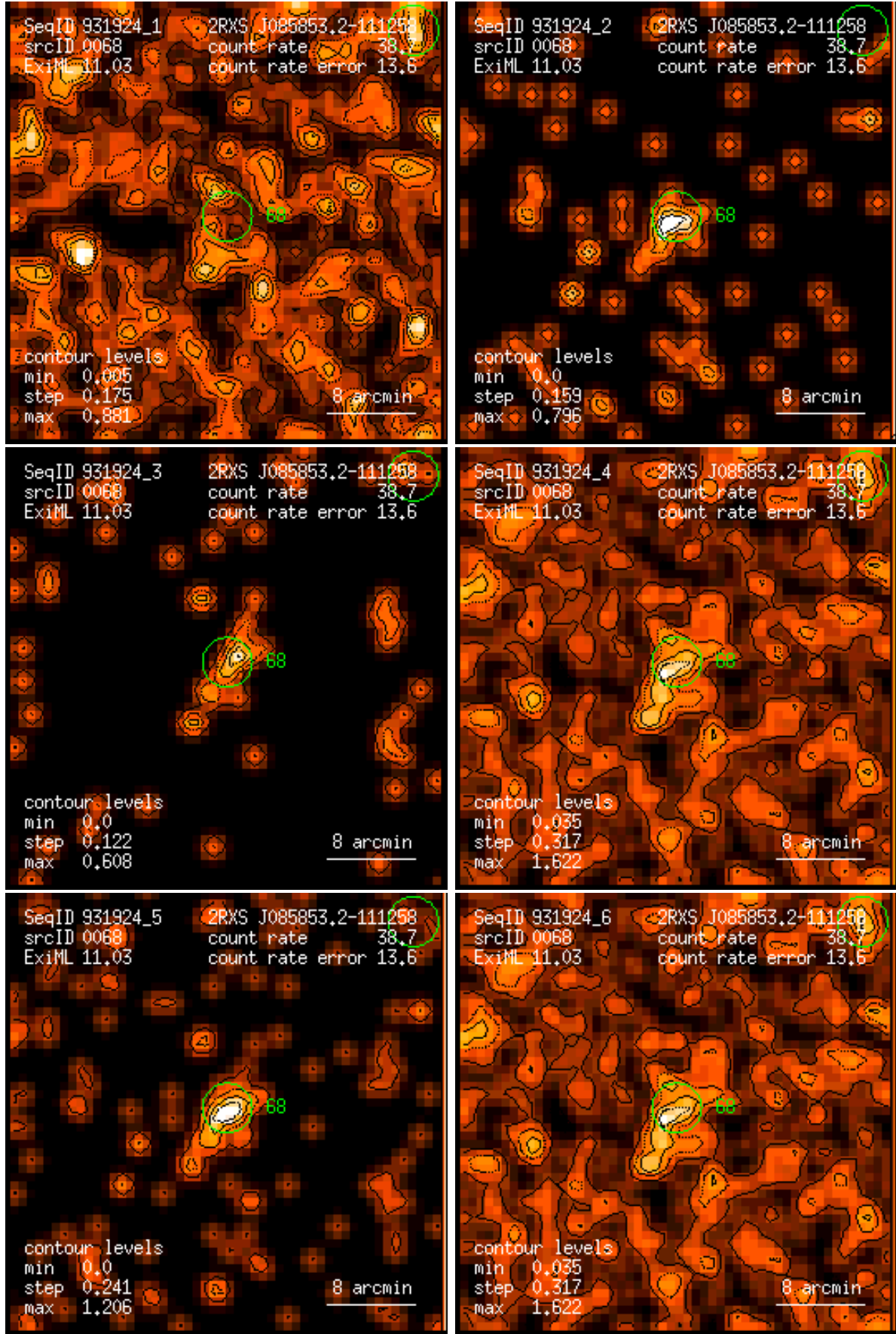
Figure 68: RASS 931924: detection 0068: band rate images, Gaussian filter: (1) PSPC channels 11 – 41, (2) 52 – 90, (3) 91 – 201, (4) 11 – 235, (5) 52 – 201, (6) 11 – 201. Broad band rates in counts/ks. Band rate contour levels in counts/ks/arcmin 2 .
