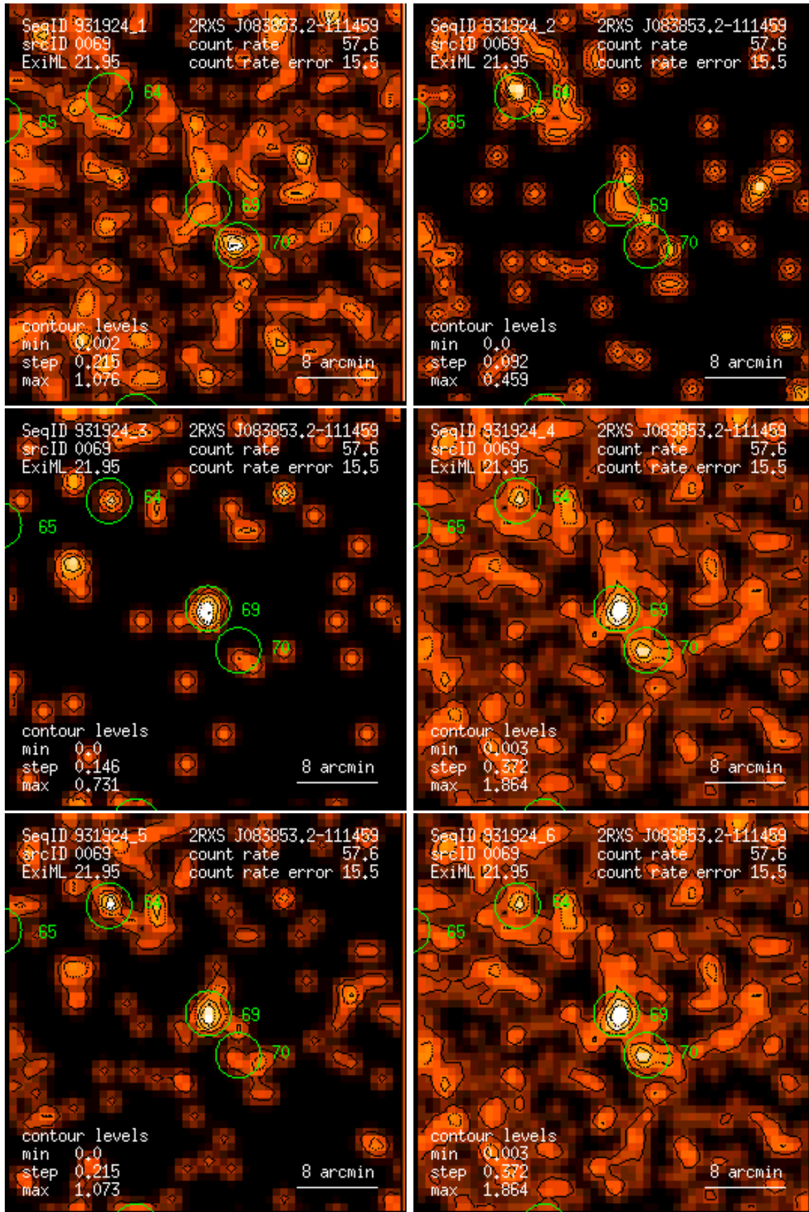
Figure 69: RASS 931924: detection 0069: band rate images, Gaussian filter: (1) PSPC channels 11 – 41, (2) 52 – 90, (3) 91 – 201, (4) 11 – 235, (5) 52 – 201, (6) 11 – 201. Broad band rates in counts/ks. Band rate contour levels in counts/ks/arcmin 2 .
