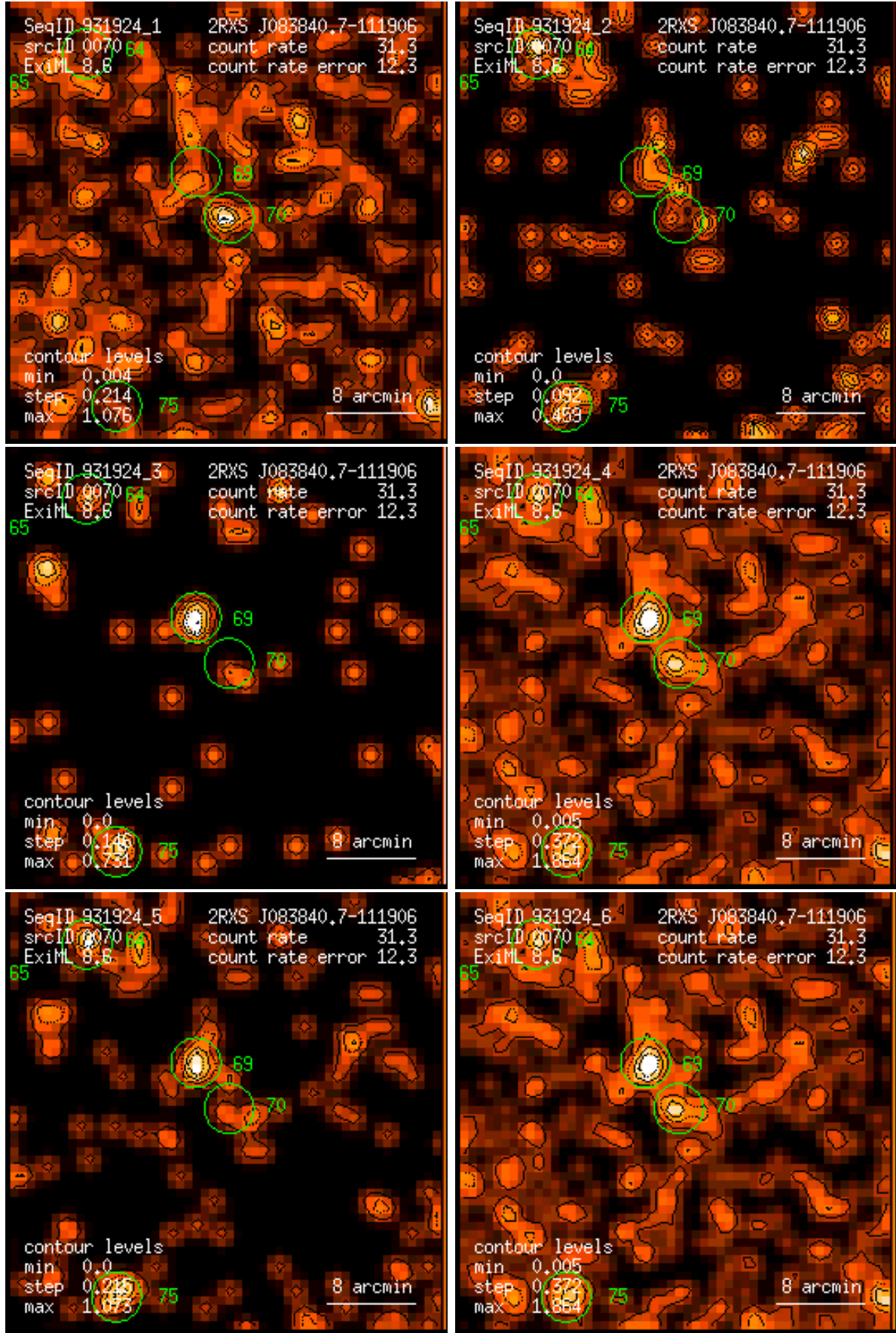
Figure 70: RASS 931924: detection 0070: band rate images, Gaussian filter: (1) PSPC channels 11 – 41, (2) 52 – 90, (3) 91 – 201, (4) 11 – 235, (5) 52 – 201, (6) 11 – 201. Broad band rates in counts/ks. Band rate contour levels in counts/ks/arcmin 2 .
