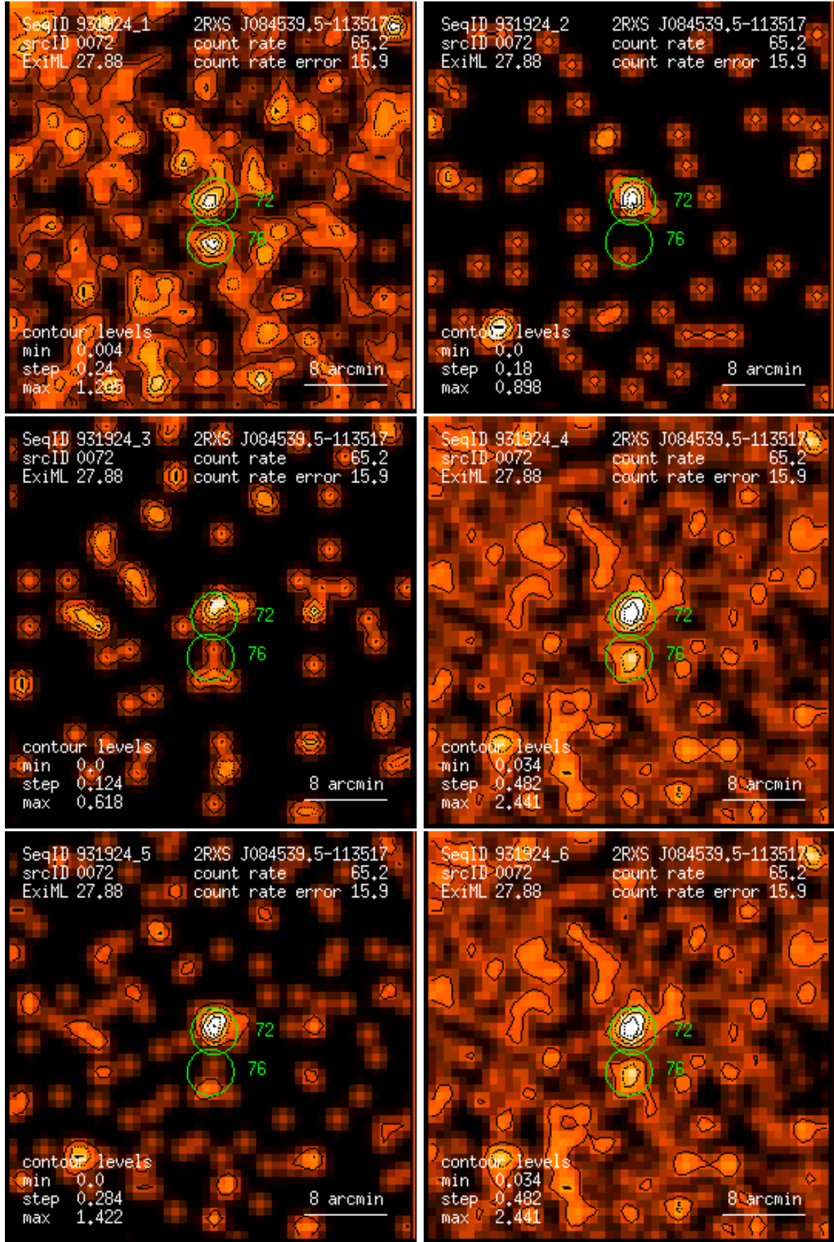
Figure 72: RASS 931924: detection 0072: band rate images, Gaussian filter: (1) PSPC channels 11 – 41, (2) 52 – 90, (3) 91 – 201, (4) 11 – 235, (5) 52 – 201, (6) 11 – 201. Broad band rates in counts/ks. Band rate contour levels in counts/ks/arcmin 2 .
