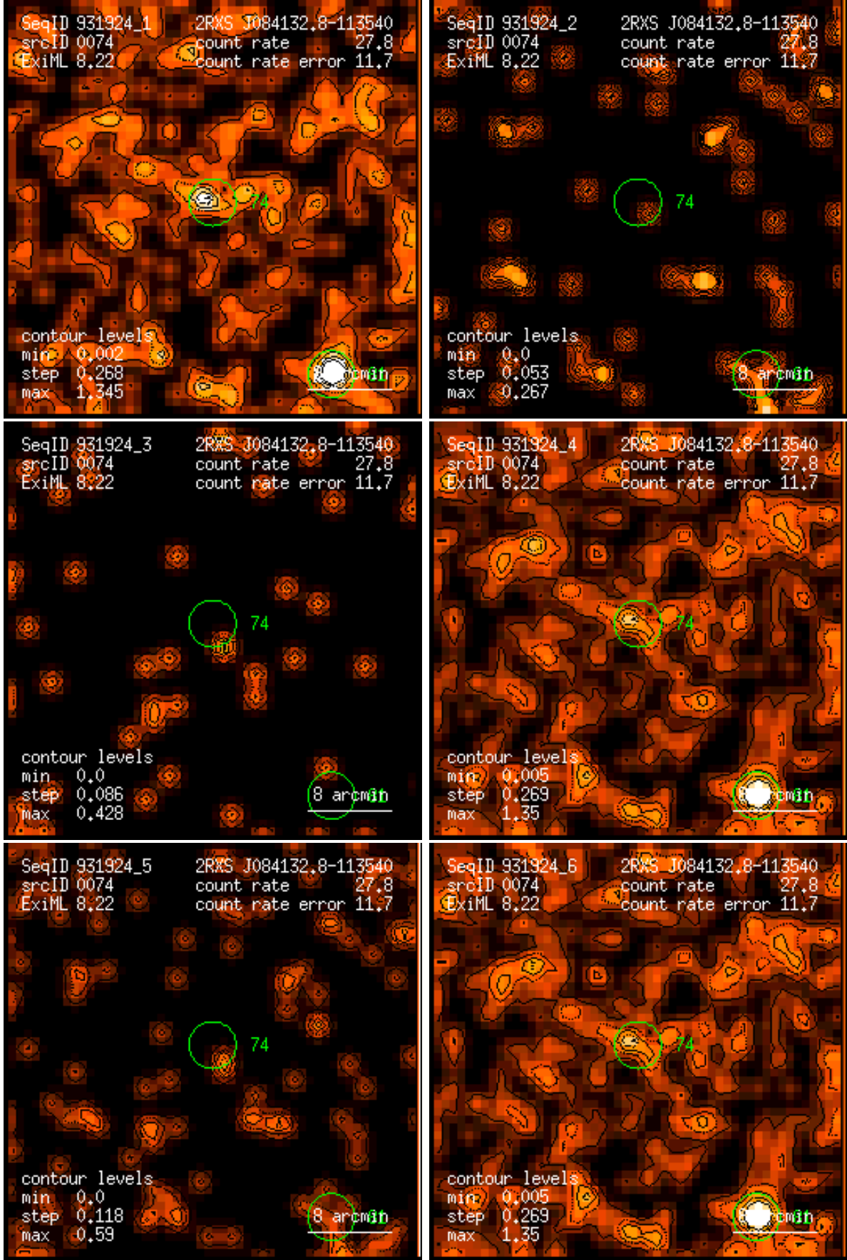
Figure 74: RASS 931924: detection 0074: band rate images, Gaussian filter: (1) PSPC channels 11 – 41, (2) 52 – 90, (3) 91 – 201, (4) 11 – 235, (5) 52 – 201, (6) 11 – 201. Broad band rates in counts/ks. Band rate contour levels in counts/ks/arcmin 2 .
