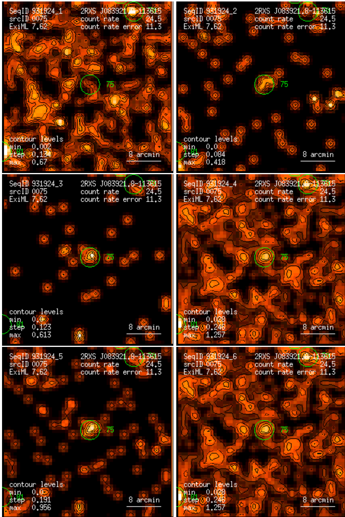
Figure 75: RASS 931924: detection 0075: band rate images, Gaussian filter: (1) PSPC channels 11 – 41, (2) 52 – 90, (3) 91 – 201, (4) 11 – 235, (5) 52 – 201, (6) 11 – 201. Broad band rates in counts/ks. Band rate contour levels in counts/ks/arcmin 2 .
