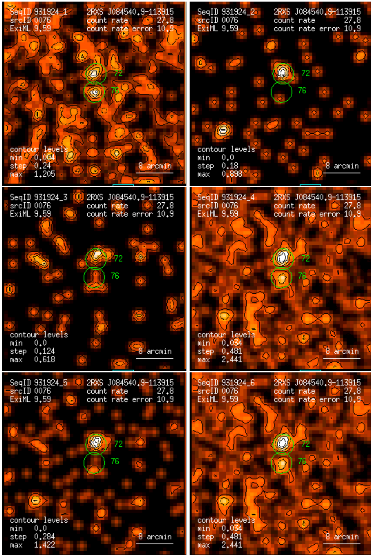
Figure 76: RASS 931924: detection 0076: band rate images, Gaussian filter: (1) PSPC channels 11 – 41, (2) 52 – 90, (3) 91 – 201, (4) 11 – 235, (5) 52 – 201, (6) 11 – 201. Broad band rates in counts/ks. Band rate contour levels in counts/ks/arcmin 2 .
