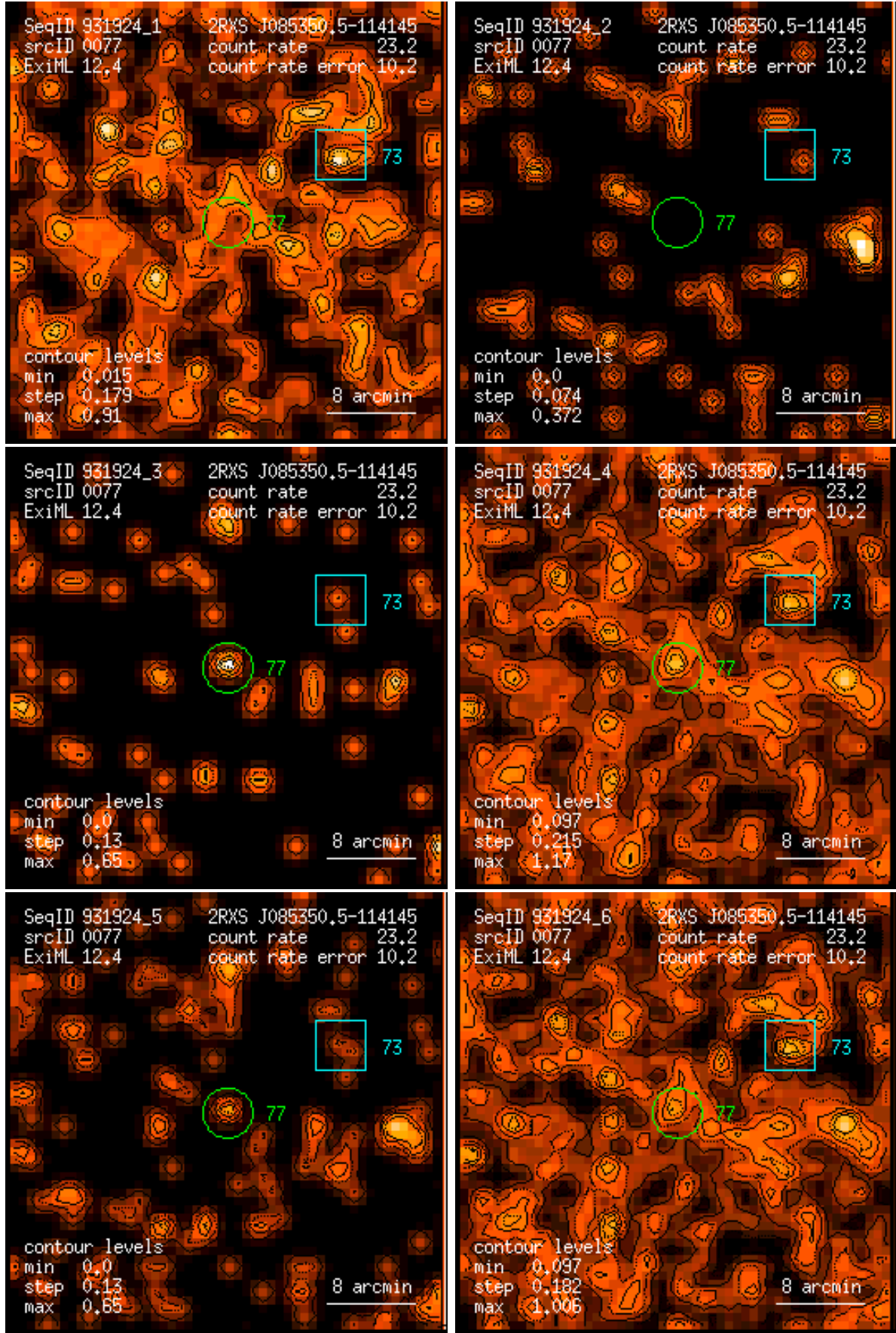
Figure 77: RASS 931924: detection 0077: band rate images, Gaussian filter: (1) PSPC channels 11 – 41, (2) 52 – 90, (3) 91 – 201, (4) 11 – 235, (5) 52 – 201, (6) 11 – 201. Broad band rates in counts/ks. Band rate contour levels in counts/ks/arcmin 2 .
