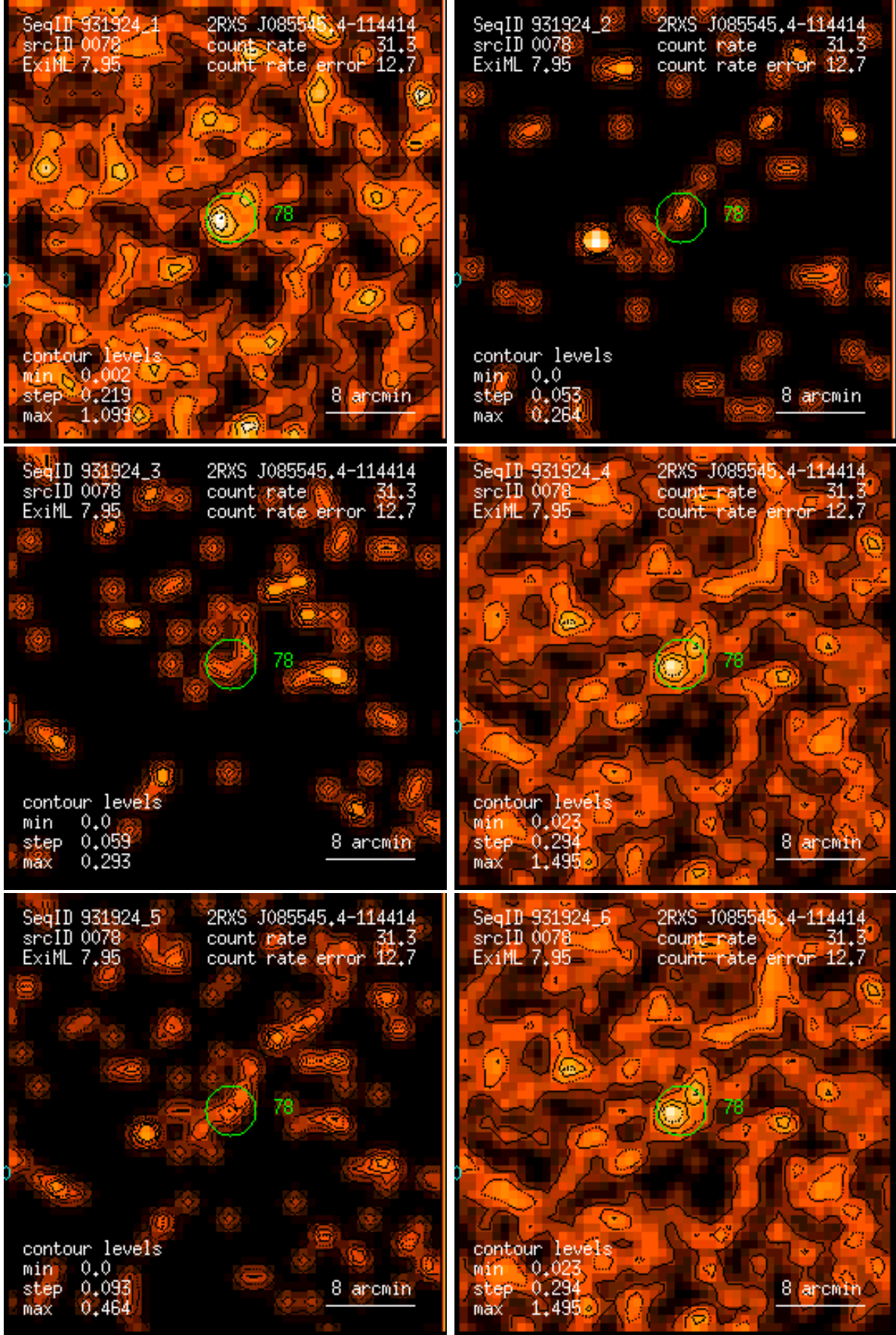
Figure 78: RASS 931924: detection 0078: band rate images, Gaussian filter: (1) PSPC channels 11 – 41, (2) 52 – 90, (3) 91 – 201, (4) 11 – 235, (5) 52 – 201, (6) 11 – 201. Broad band rates in counts/ks. Band rate contour levels in counts/ks/arcmin 2 .
