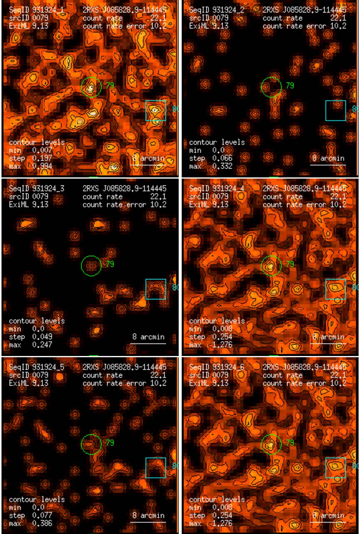
Figure 79: RASS 931924: detection 0079: band rate images, Gaussian filter: (1) PSPC channels 11 – 41, (2) 52 – 90, (3) 91 – 201, (4) 11 – 235, (5) 52 – 201, (6) 11 – 201. Broad band rates in counts/ks. Band rate contour levels in counts/ks/arcmin 2 .
