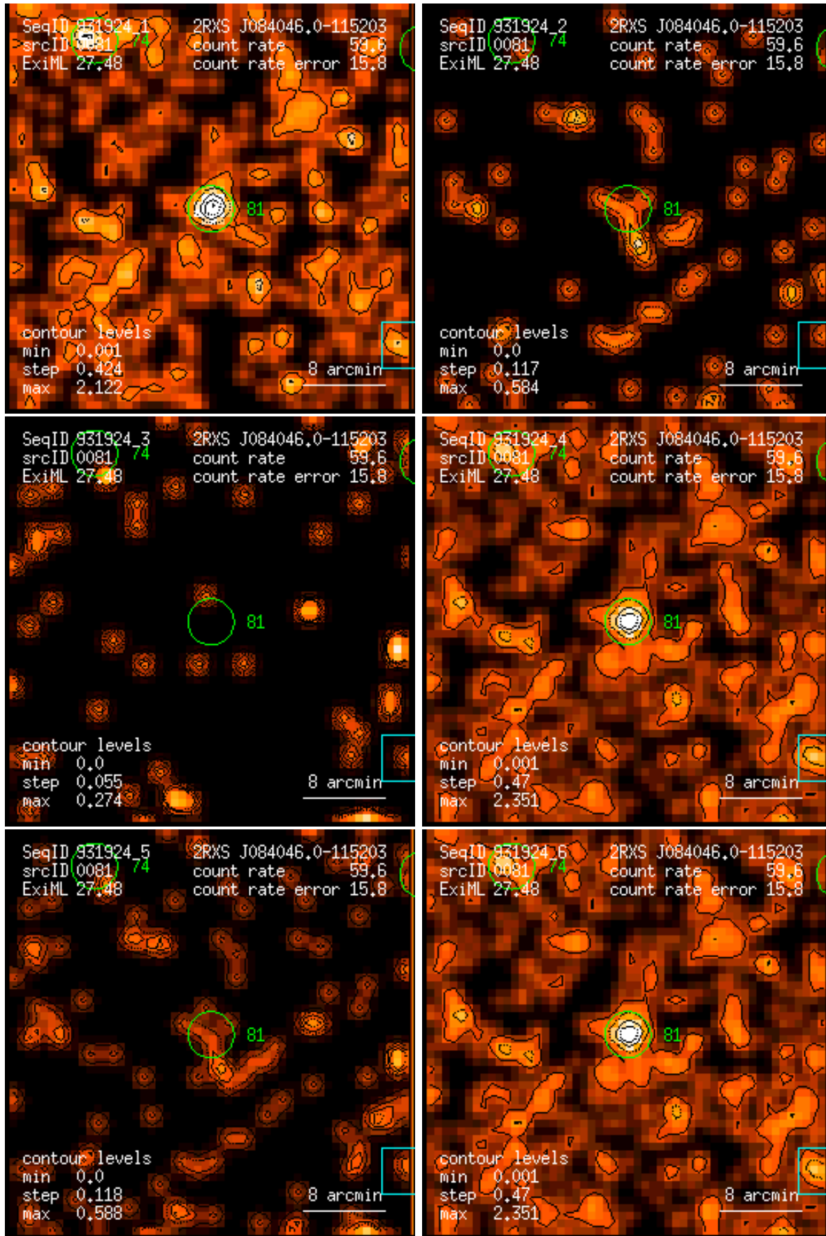
Figure 81: RASS 931924: detection 0081: band rate images, Gaussian filter: (1) PSPC channels 11 – 41, (2) 52 – 90, (3) 91 – 201, (4) 11 – 235, (5) 52 – 201, (6) 11 – 201. Broad band rates in counts/ks. Band rate contour levels in counts/ks/arcmin 2 .
