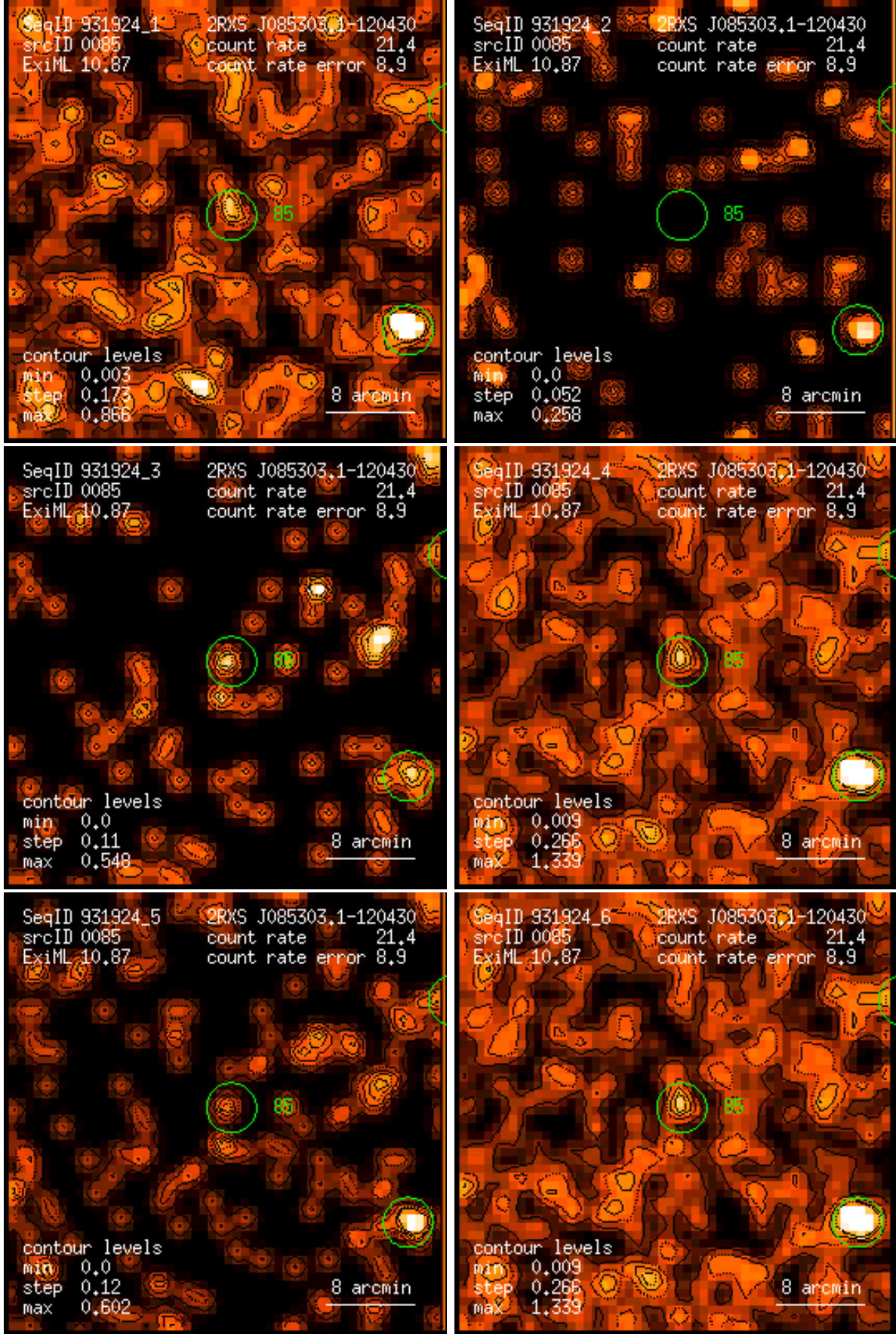
Figure 85: RASS 931924: detection 0085: band rate images, Gaussian filter: (1) PSPC channels 11 – 41, (2) 52 – 90, (3) 91 – 201, (4) 11 – 235, (5) 52 – 201, (6) 11 – 201. Broad band rates in counts/ks. Band rate contour levels in counts/ks/arcmin 2 .
