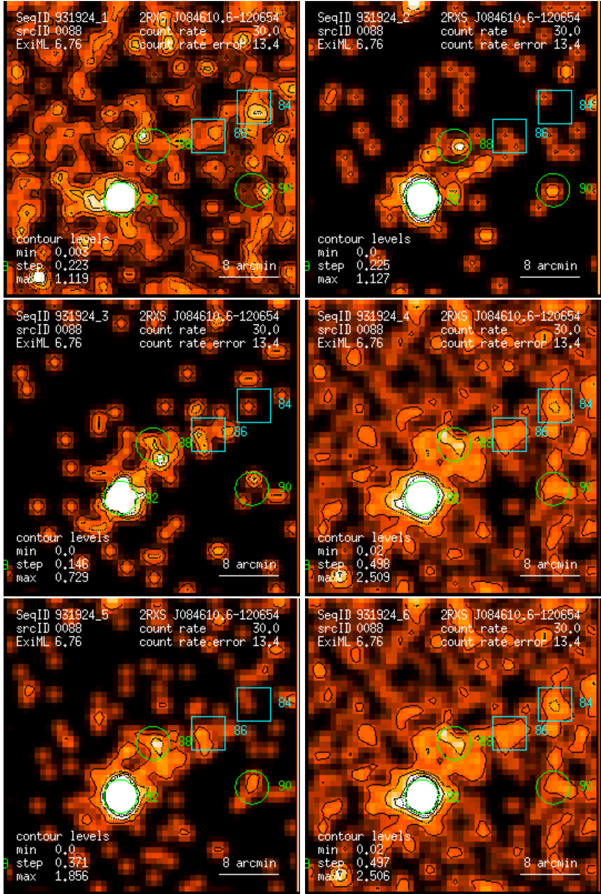
Figure 88: RASS 931924: detection 0088: band rate images, Gaussian filter: (1) PSPC channels 11 – 41, (2) 52 – 90, (3) 91 – 201, (4) 11 – 235, (5) 52 – 201, (6) 11 – 201. Broad band rates in counts/ks. Band rate contour levels in counts/ks/arcmin 2 .
