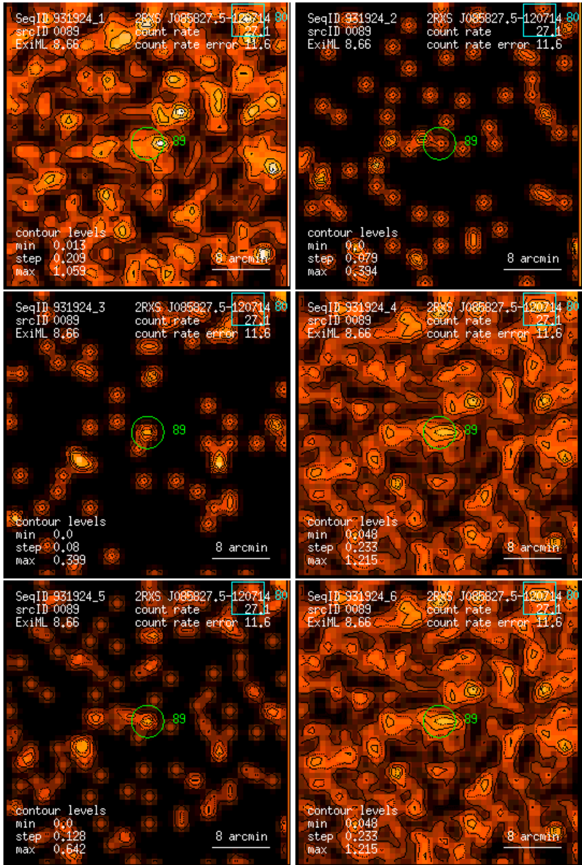
Figure 89: RASS 931924: detection 0089: band rate images, Gaussian filter: (1) PSPC channels 11 – 41, (2) 52 – 90, (3) 91 – 201, (4) 11 – 235, (5) 52 – 201, (6) 11 – 201. Broad band rates in counts/ks. Band rate contour levels in counts/ks/arcmin 2 .
