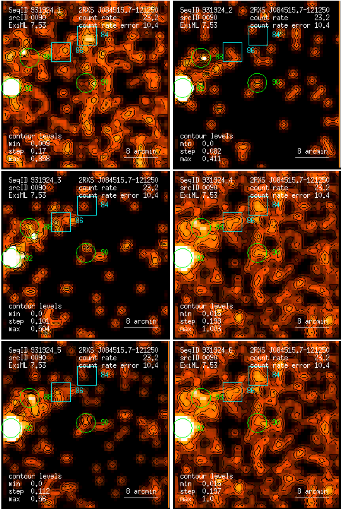
Figure 90: RASS 931924: detection 0090: band rate images, Gaussian filter: (1) PSPC channels 11 – 41, (2) 52 – 90, (3) 91 – 201, (4) 11 – 235, (5) 52 – 201, (6) 11 – 201. Broad band rates in counts/ks. Band rate contour levels in counts/ks/arcmin 2 .
