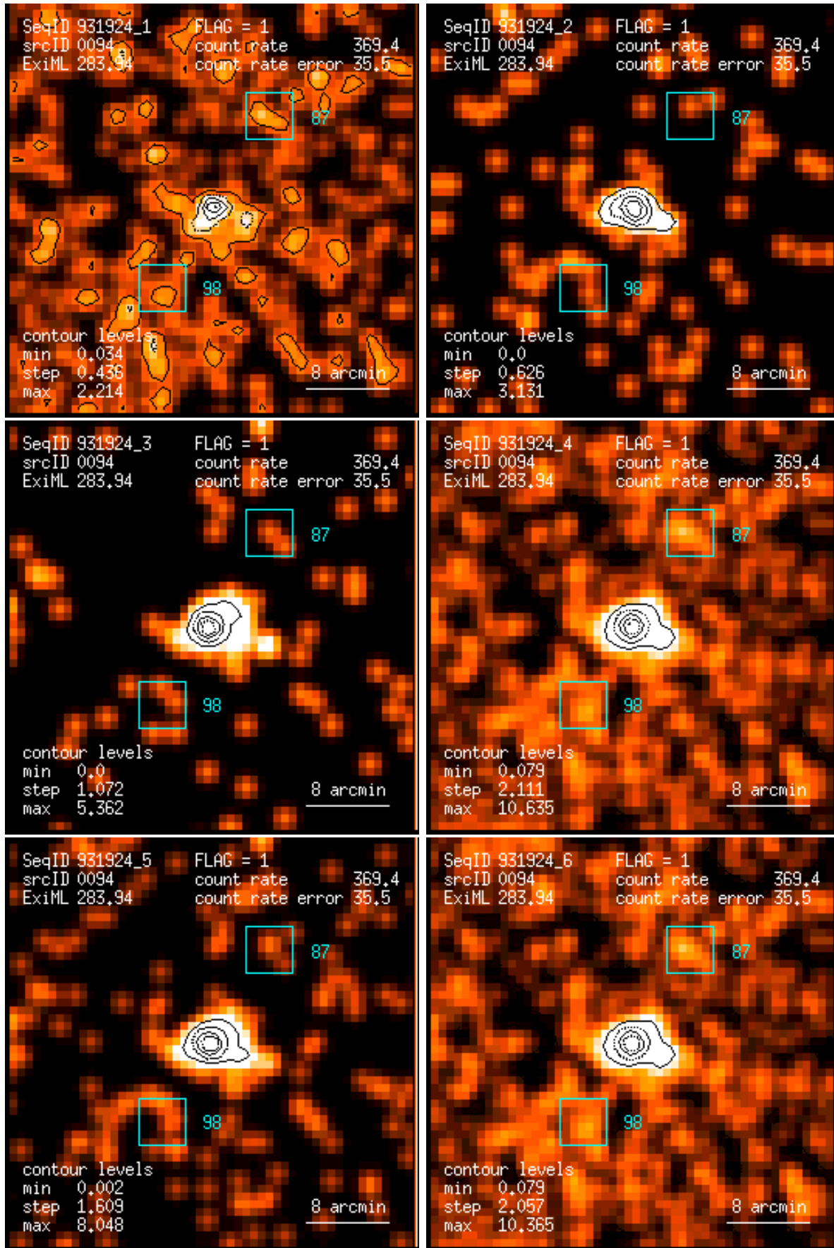
Figure 94: RASS 931924: detection 0094: band rate images, Gaussian filter: (1) PSPC channels 11 – 41, (2) 52 – 90, (3) 91 – 201, (4) 11 – 235, (5) 52 – 201, (6) 11 – 201. Broad band rates in counts/ks. Band rate contour levels in counts/ks/arcmin 2 .
