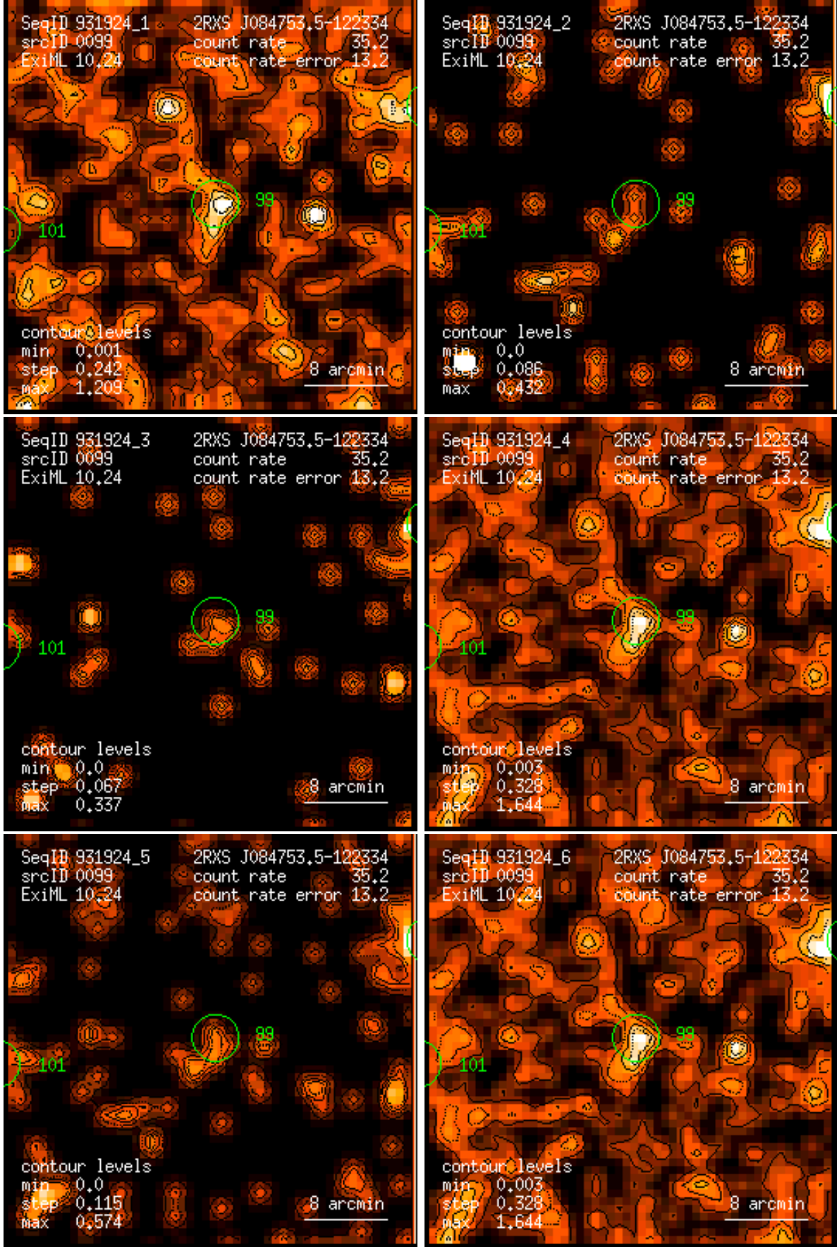
Figure 99: RASS 931924: detection 0099: band rate images, Gaussian filter: (1) PSPC channels 11 – 41, (2) 52 – 90, (3) 91 – 201, (4) 11 – 235, (5) 52 – 201, (6) 11 – 201. Broad band rates in counts/ks. Band rate contour levels in counts/ks/arcmin 2 .
