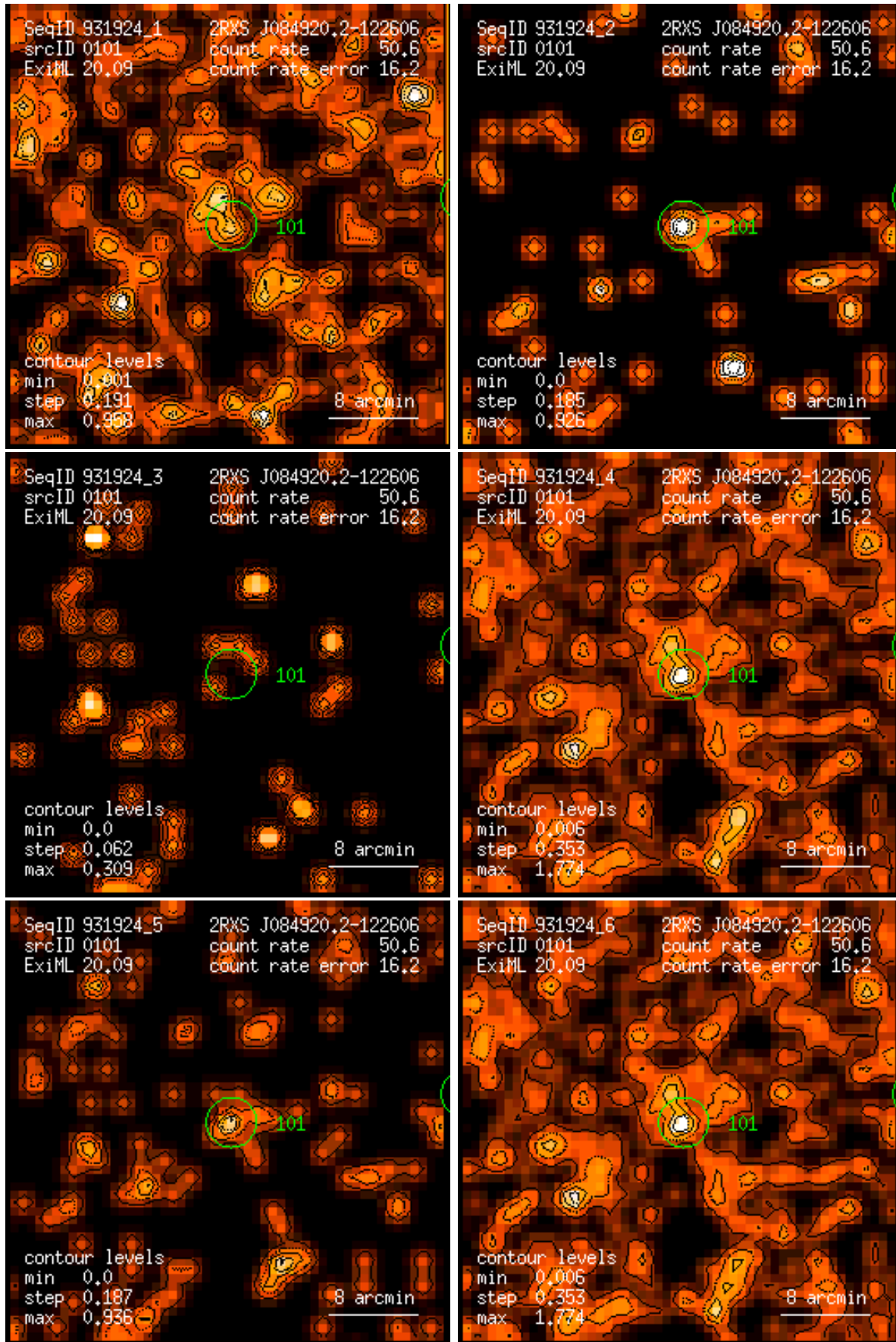
Figure 101: RASS 931924: detection 0101: band rate images, Gaussian filter: (1) PSPC channels 11 – 41, (2) 52 – 90, (3) 91 – 201, (4) 11 – 235, (5) 52 – 201, (6) 11 – 201. Broad band rates in counts/ks. Band rate contour levels in counts/ks/arcmin 2 .
