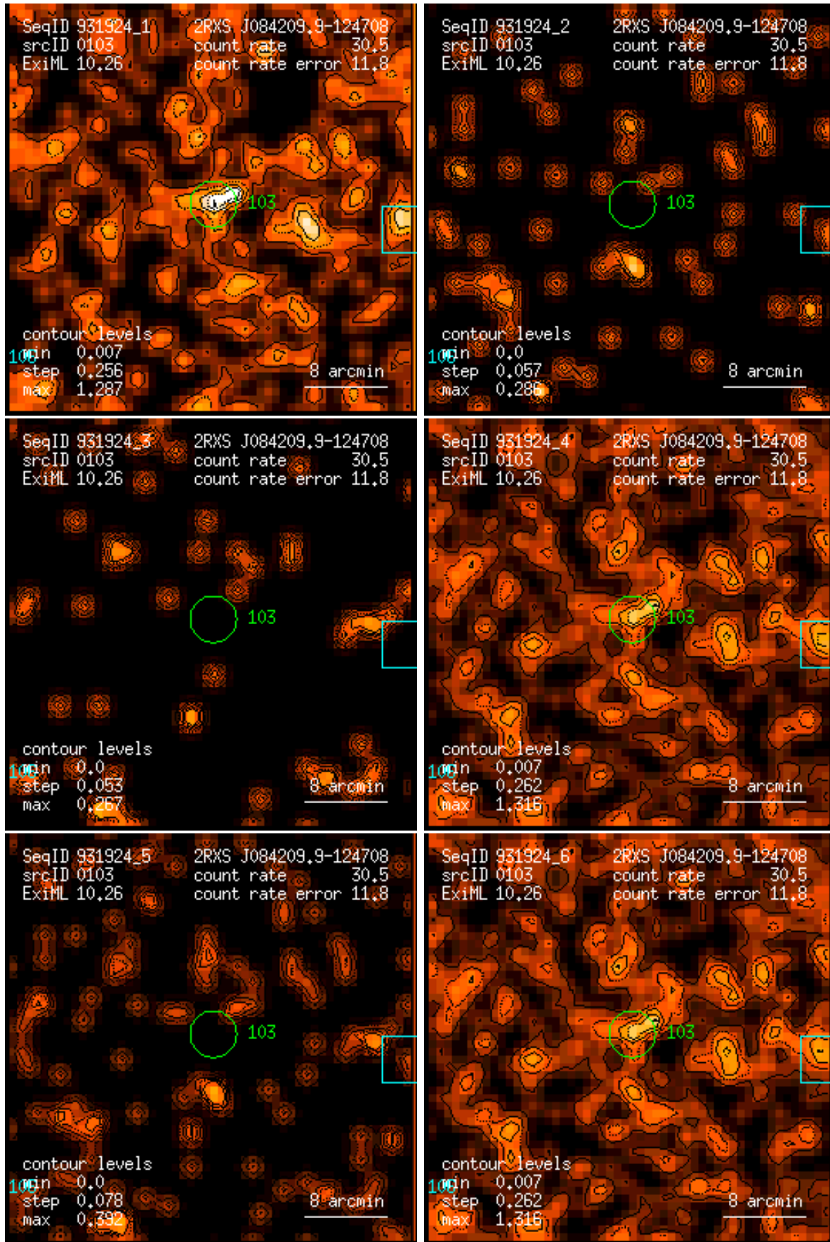
Figure 103: RASS 931924: detection 0103: band rate images, Gaussian filter: (1) PSPC channels 11 – 41, (2) 52 – 90, (3) 91 – 201, (4) 11 – 235, (5) 52 – 201, (6) 11 – 201. Broad band rates in counts/ks. Band rate contour levels in counts/ks/arcmin 2 .
