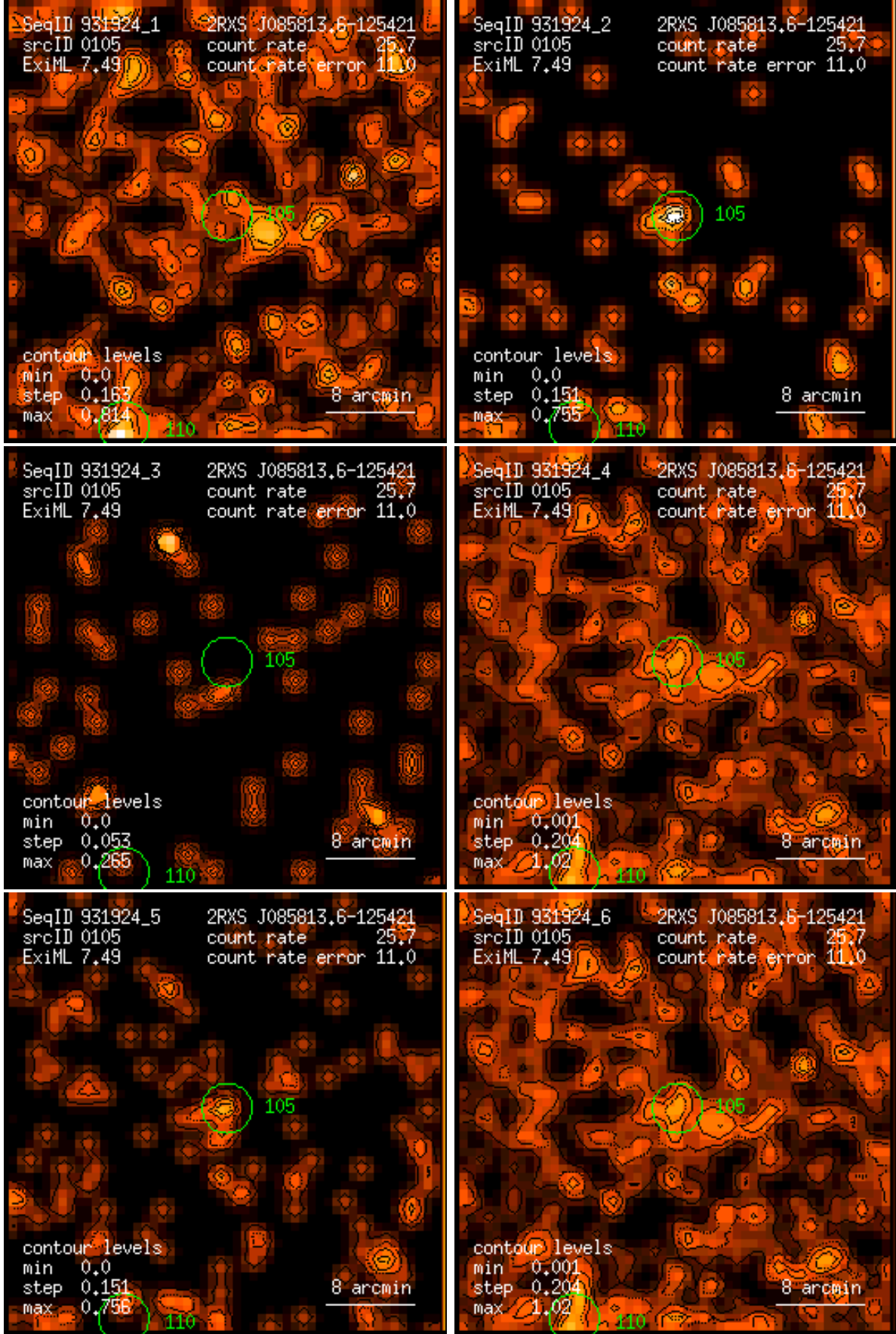
Figure 105: RASS 931924: detection 0105: band rate images, Gaussian filter: (1) PSPC channels 11 – 41, (2) 52 – 90, (3) 91 – 201, (4) 11 – 235, (5) 52 – 201, (6) 11 – 201. Broad band rates in counts/ks. Band rate contour levels in counts/ks/arcmin 2 .
