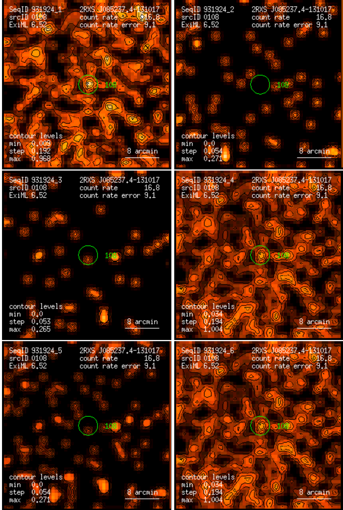
Figure 108: RASS 931924: detection 0108: band rate images, Gaussian filter: (1) PSPC channels 11 – 41, (2) 52 – 90, (3) 91 – 201, (4) 11 – 235, (5) 52 – 201, (6) 11 – 201. Broad band rates in counts/ks. Band rate contour levels in counts/ks/arcmin 2 .
