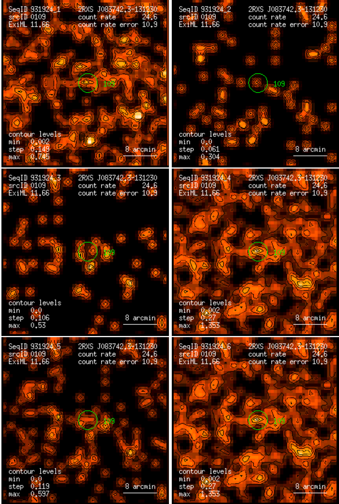
Figure 109: RASS 931924: detection 0109: band rate images, Gaussian filter: (1) PSPC channels 11 – 41, (2) 52 – 90, (3) 91 – 201, (4) 11 – 235, (5) 52 – 201, (6) 11 – 201. Broad band rates in counts/ks. Band rate contour levels in counts/ks/arcmin 2 .
