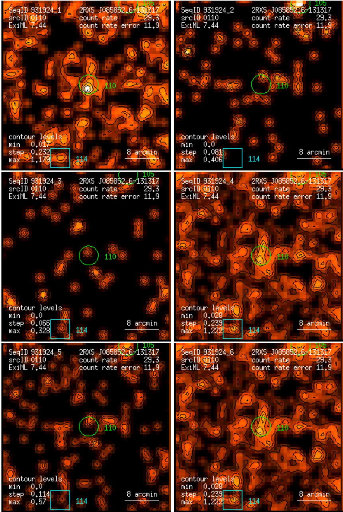
Figure 110: RASS 931924: detection 0110: band rate images, Gaussian filter: (1) PSPC channels 11 – 41, (2) 52 – 90, (3) 91 – 201, (4) 11 – 235, (5) 52 – 201, (6) 11 – 201. Broad band rates in counts/ks. Band rate contour levels in counts/ks/arcmin 2 .
