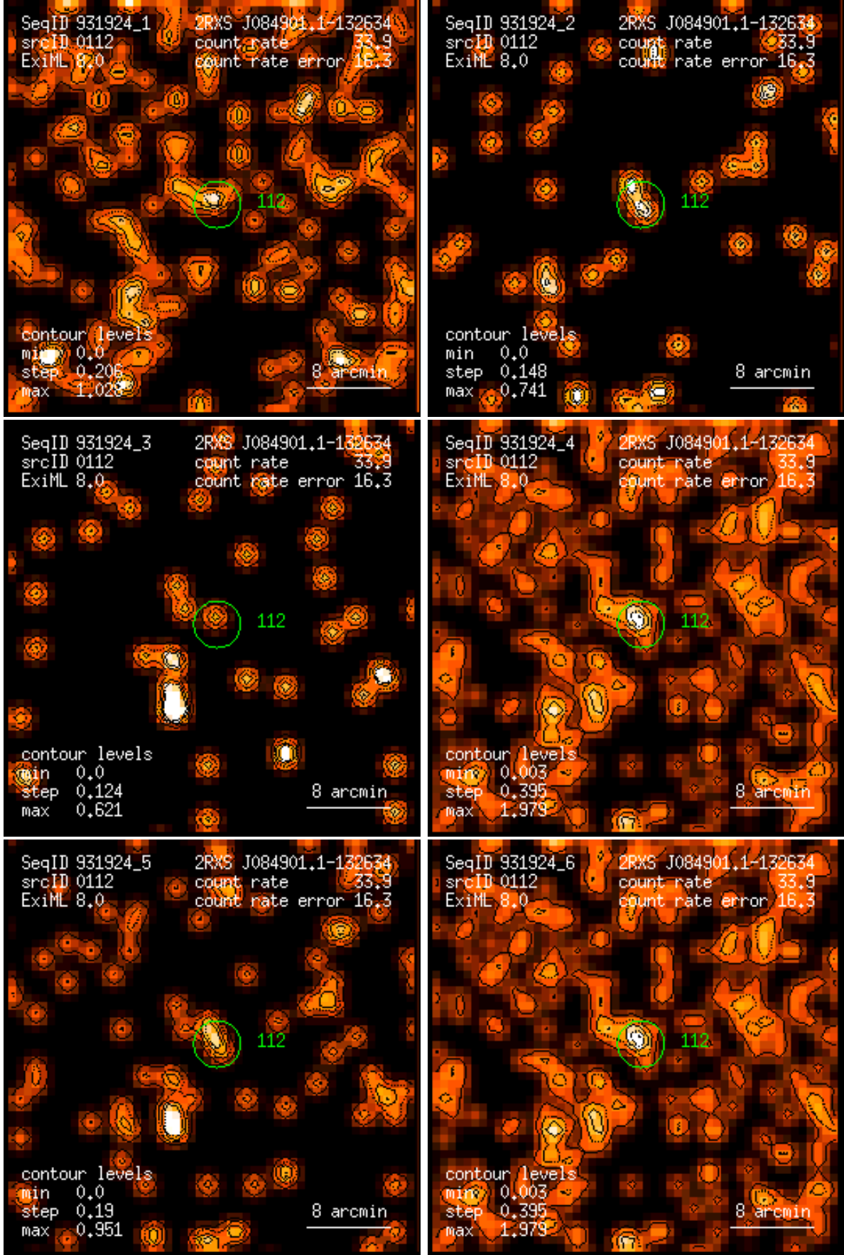
Figure 112: RASS 931924: detection 0112: band rate images, Gaussian filter: (1) PSPC channels 11 – 41, (2) 52 – 90, (3) 91 – 201, (4) 11 – 235, (5) 52 – 201, (6) 11 – 201. Broad band rates in counts/ks. Band rate contour levels in counts/ks/arcmin 2 .
