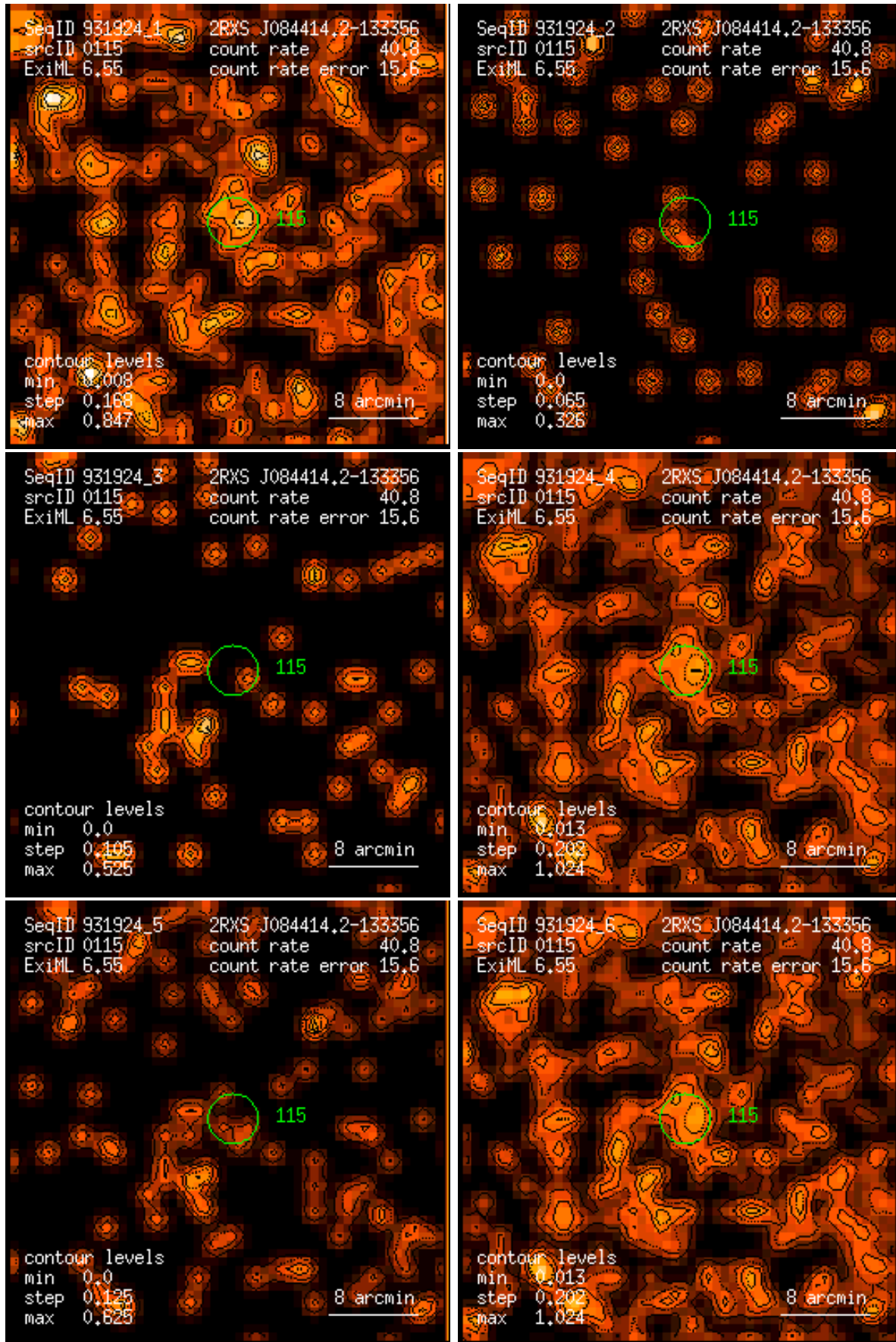
Figure 115: RASS 931924: detection 0115: band rate images, Gaussian filter: (1) PSPC channels 11 – 41, (2) 52 – 90, (3) 91 – 201, (4) 11 – 235, (5) 52 – 201, (6) 11 – 201. Broad band rates in counts/ks. Band rate contour levels in counts/ks/arcmin 2 .
