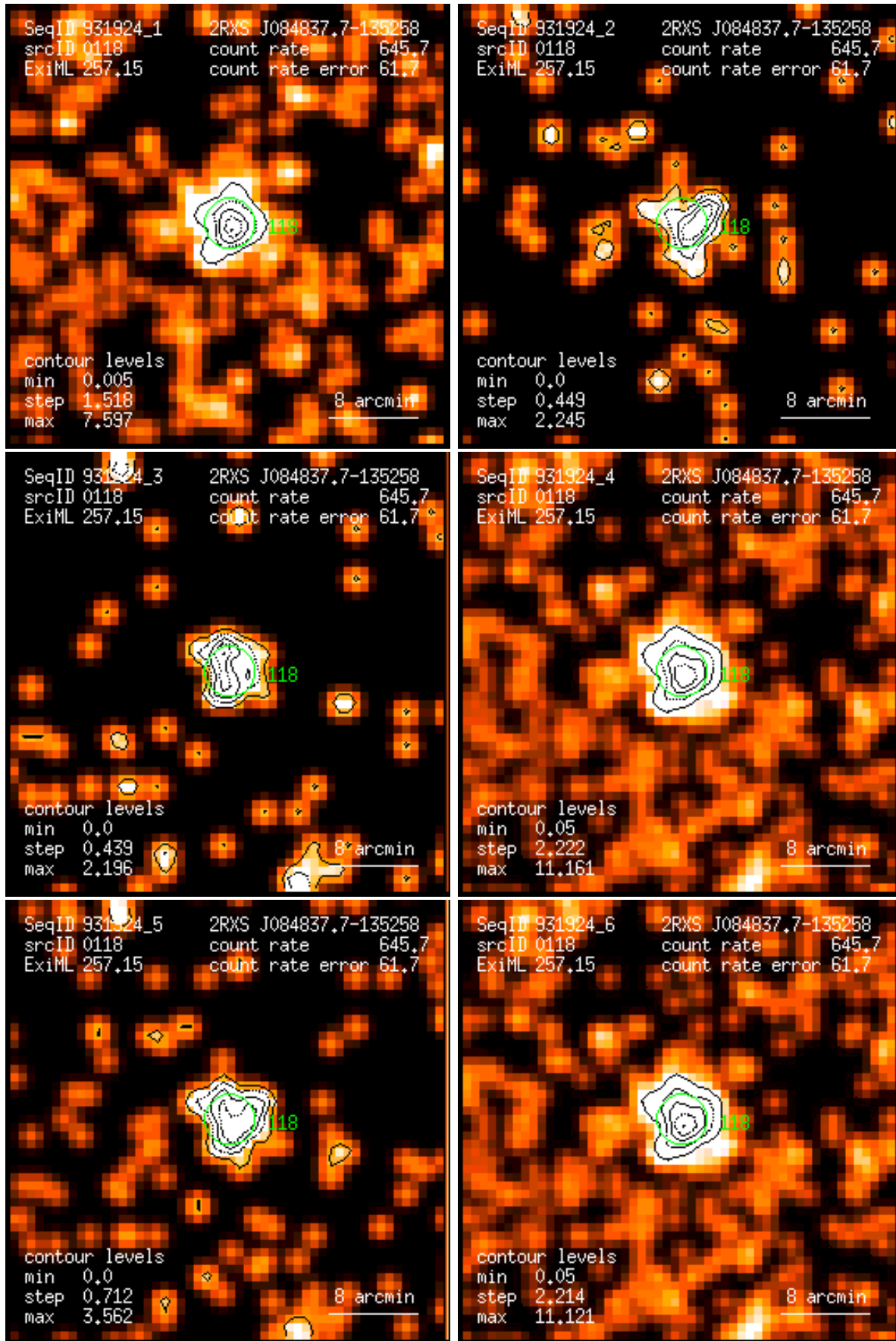
Figure 118: RASS 931924: detection 0118: band rate images, Gaussian filter: (1) PSPC channels 11 – 41, (2) 52 – 90, (3) 91 – 201, (4) 11 – 235, (5) 52 – 201, (6) 11 – 201. Broad band rates in counts/ks. Band rate contour levels in counts/ks/arcmin 2 .
