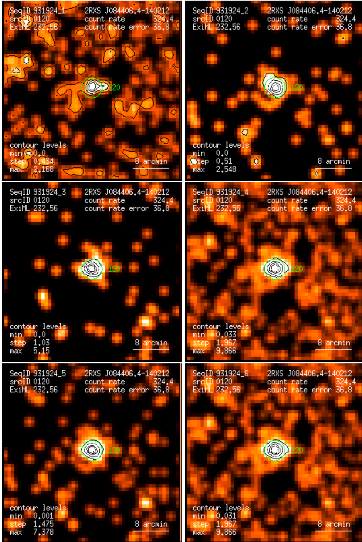
Figure 120: RASS 931924: detection 0120: band rate images, Gaussian filter: (1) PSPC channels 11 – 41, (2) 52 – 90, (3) 91 – 201, (4) 11 – 235, (5) 52 – 201, (6) 11 – 201. Broad band rates in counts/ks. Band rate contour levels in counts/ks/arcmin 2 .
