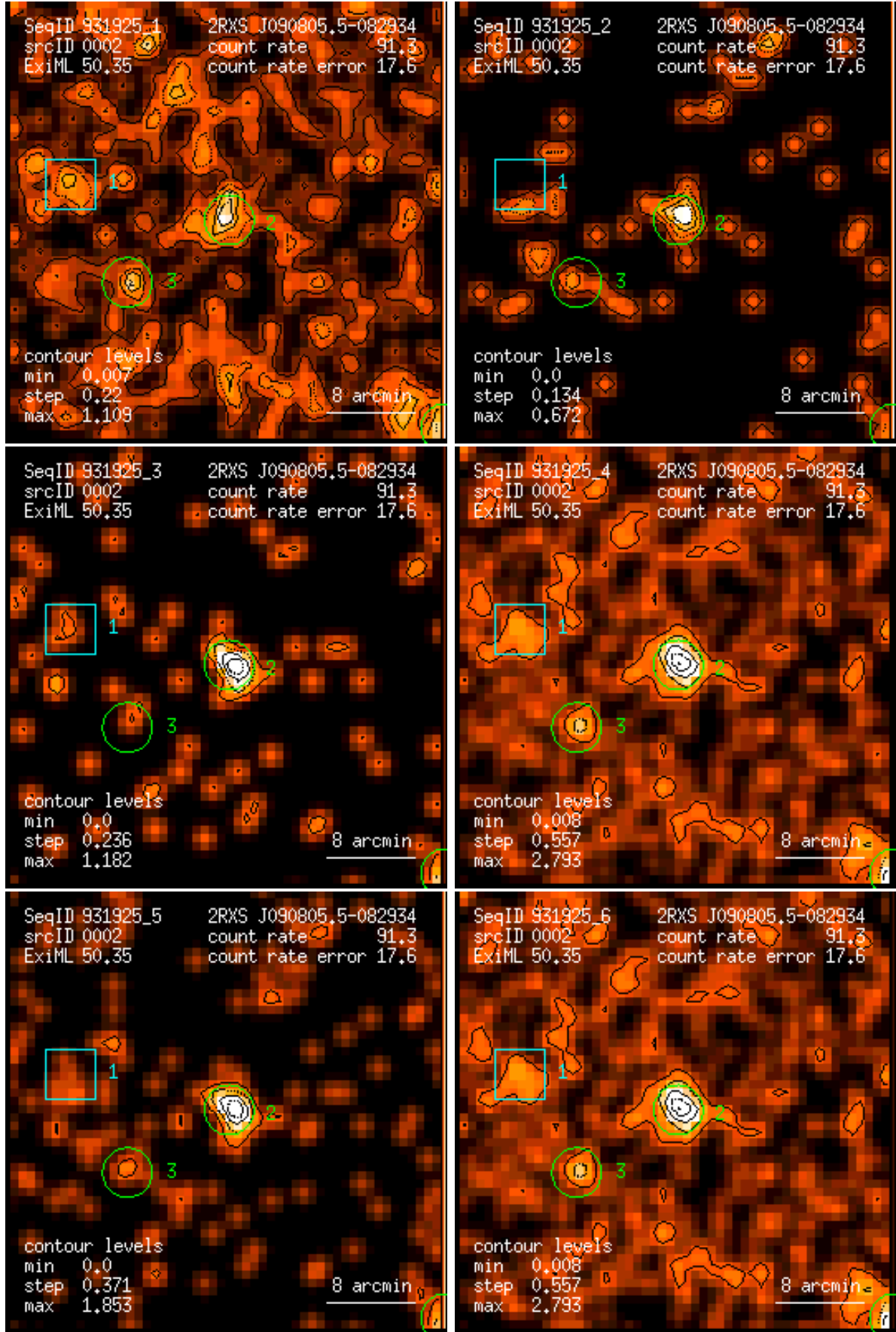
Figure 2: RASS 931925: detection 0002: band rate images, Gaussian filter: (1) PSPC channels 11 – 41, (2) 52 – 90, (3) 91 – 201, (4) 11 – 235, (5) 52 – 201, (6) 11 – 201. Broad band rates in counts/ks. Band rate contour levels in counts/ks/arcmin 2 .
