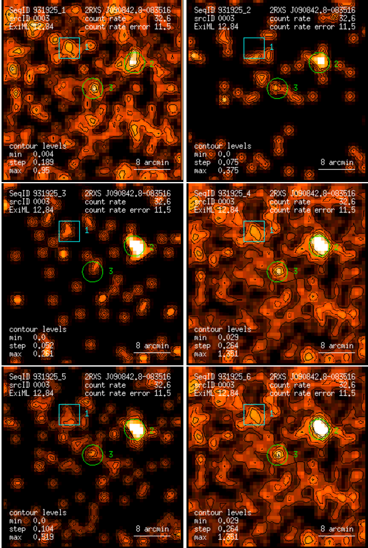
Figure 3: RASS 931925: detection 0003: band rate images, Gaussian filter: (1) PSPC channels 11 – 41, (2) 52 – 90, (3) 91 – 201, (4) 11 – 235, (5) 52 – 201, (6) 11 – 201. Broad band rates in counts/ks. Band rate contour levels in counts/ks/arcmin 2 .
