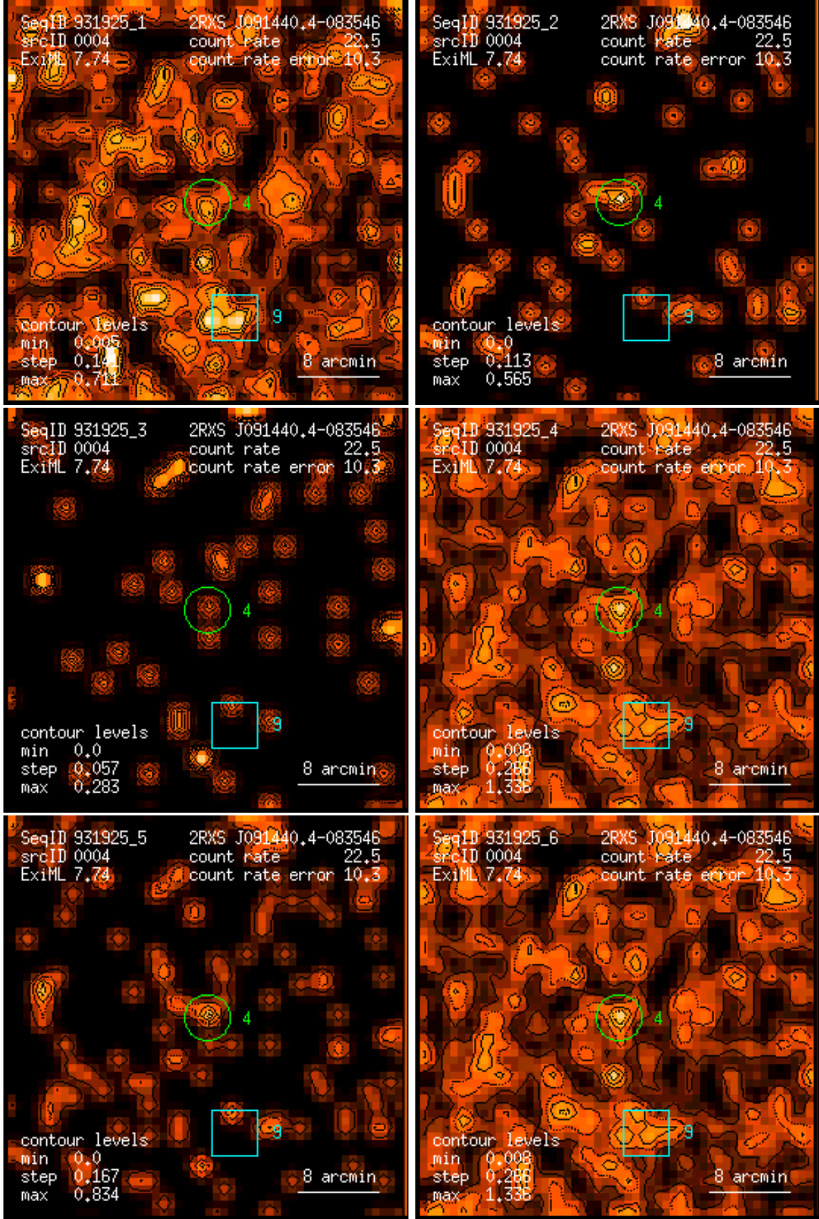
Figure 4: RASS 931925: detection 0004: band rate images, Gaussian filter: (1) PSPC channels 11 – 41, (2) 52 – 90, (3) 91 – 201, (4) 11 – 235, (5) 52 – 201, (6) 11 – 201. Broad band rates in counts/ks. Band rate contour levels in counts/ks/arcmin 2 .
