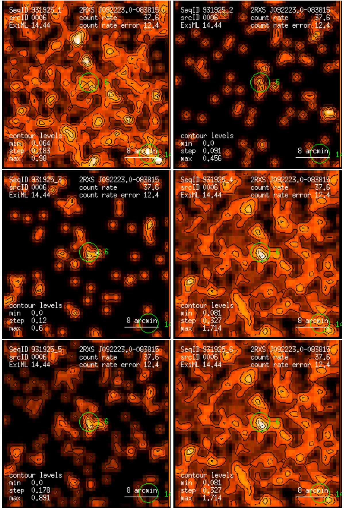
Figure 6: RASS 931925: detection 0006: band rate images, Gaussian filter: (1) PSPC channels 11 – 41, (2) 52 – 90, (3) 91 – 201, (4) 11 – 235, (5) 52 – 201, (6) 11 – 201. Broad band rates in counts/ks. Band rate contour levels in counts/ks/arcmin 2 .
