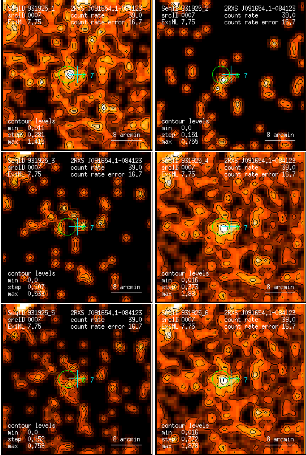
Figure 7: RASS 931925: detection 0007: band rate images, Gaussian filter: (1) PSPC channels 11 – 41, (2) 52 – 90, (3) 91 – 201, (4) 11 – 235, (5) 52 – 201, (6) 11 – 201. Broad band rates in counts/ks. Band rate contour levels in counts/ks/arcmin 2 .
