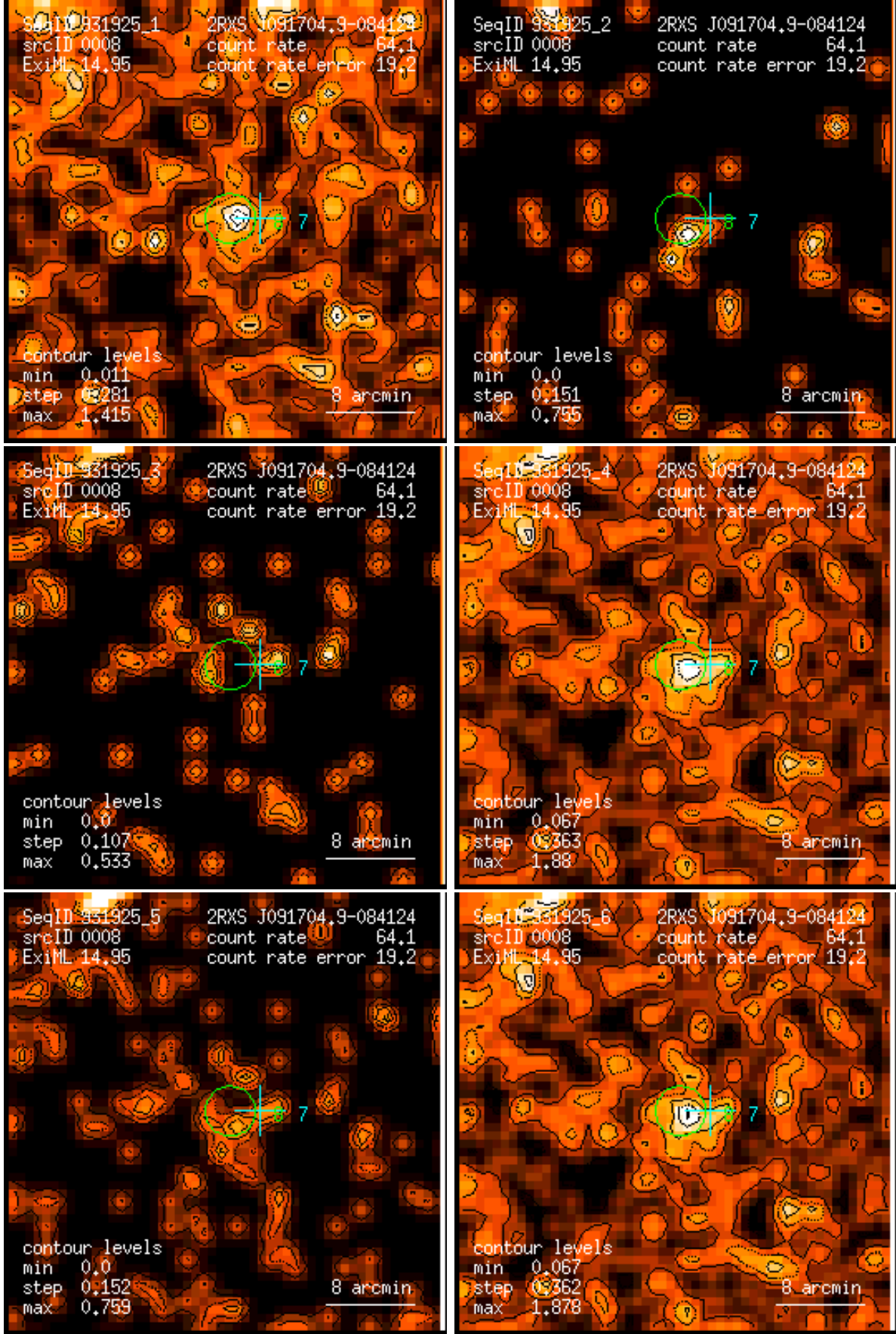
Figure 8: RASS 931925: detection 0008: band rate images, Gaussian filter: (1) PSPC channels 11 – 41, (2) 52 – 90, (3) 91 – 201, (4) 11 – 235, (5) 52 – 201, (6) 11 – 201. Broad band rates in counts/ks. Band rate contour levels in counts/ks/arcmin 2 .
