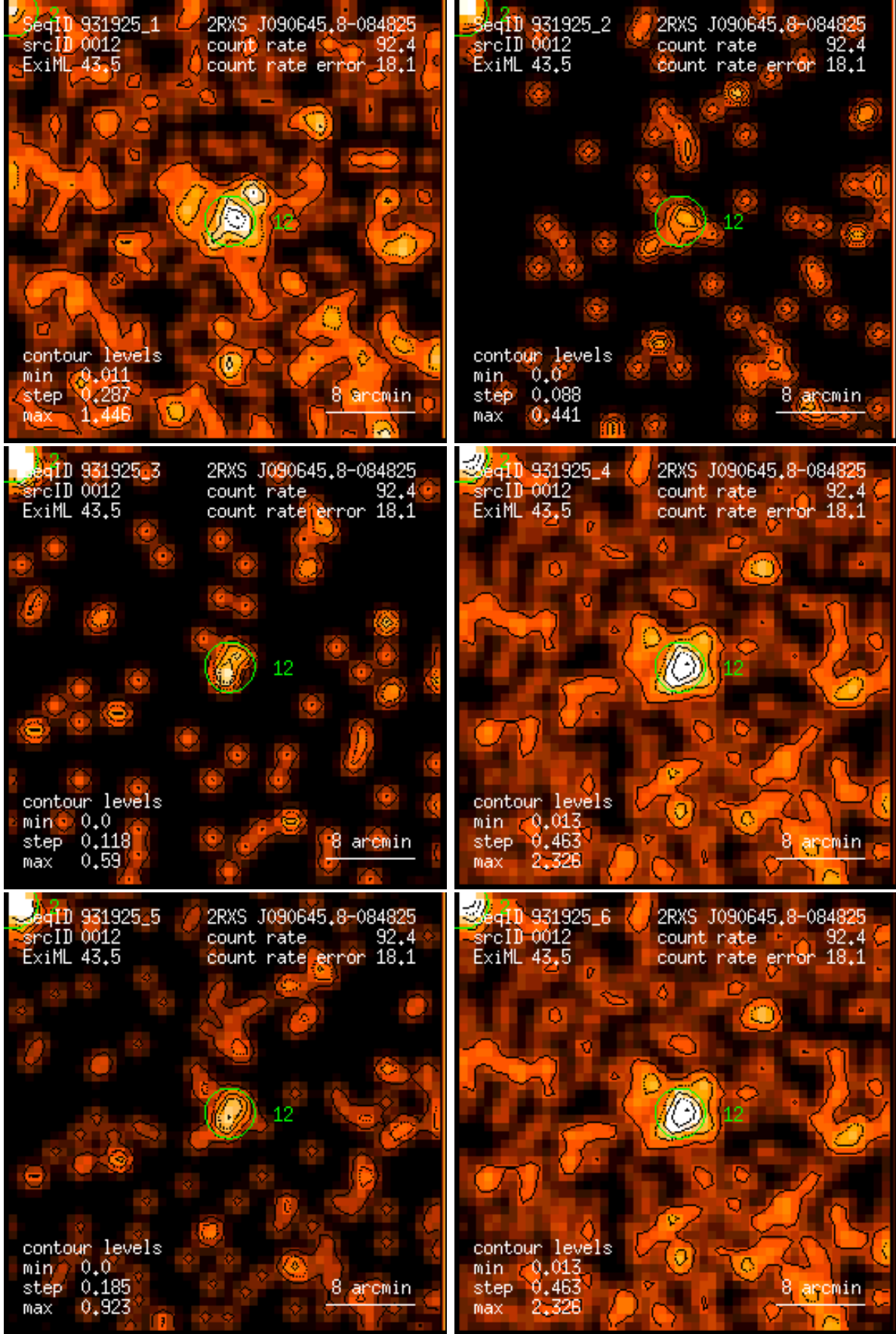
Figure 12: RASS 931925: detection 0012: band rate images, Gaussian filter: (1) PSPC channels 11 – 41, (2) 52 – 90, (3) 91 – 201, (4) 11 – 235, (5) 52 – 201, (6) 11 – 201. Broad band rates in counts/ks. Band rate contour levels in counts/ks/arcmin 2 .
