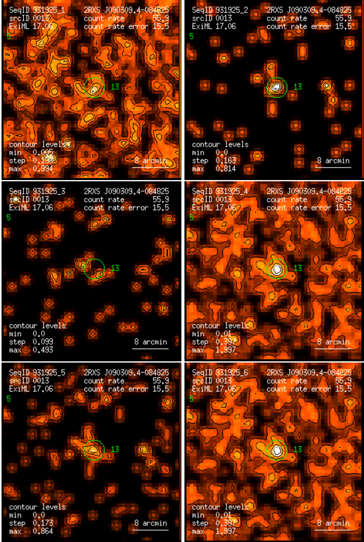
Figure 13: RASS 931925: detection 0013: band rate images, Gaussian filter: (1) PSPC channels 11 – 41, (2) 52 – 90, (3) 91 – 201, (4) 11 – 235, (5) 52 – 201, (6) 11 – 201. Broad band rates in counts/ks. Band rate contour levels in counts/ks/arcmin 2 .
