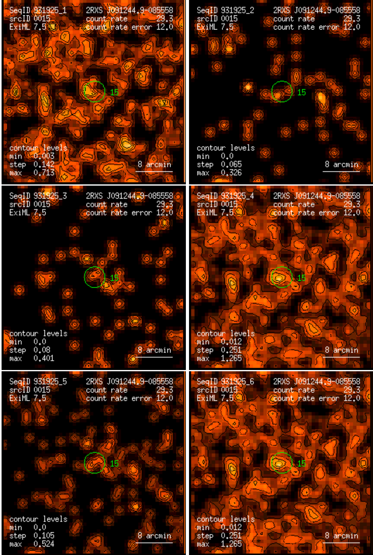
Figure 15: RASS 931925: detection 0015: band rate images, Gaussian filter: (1) PSPC channels 11 – 41, (2) 52 – 90, (3) 91 – 201, (4) 11 – 235, (5) 52 – 201, (6) 11 – 201. Broad band rates in counts/ks. Band rate contour levels in counts/ks/arcmin 2 .
