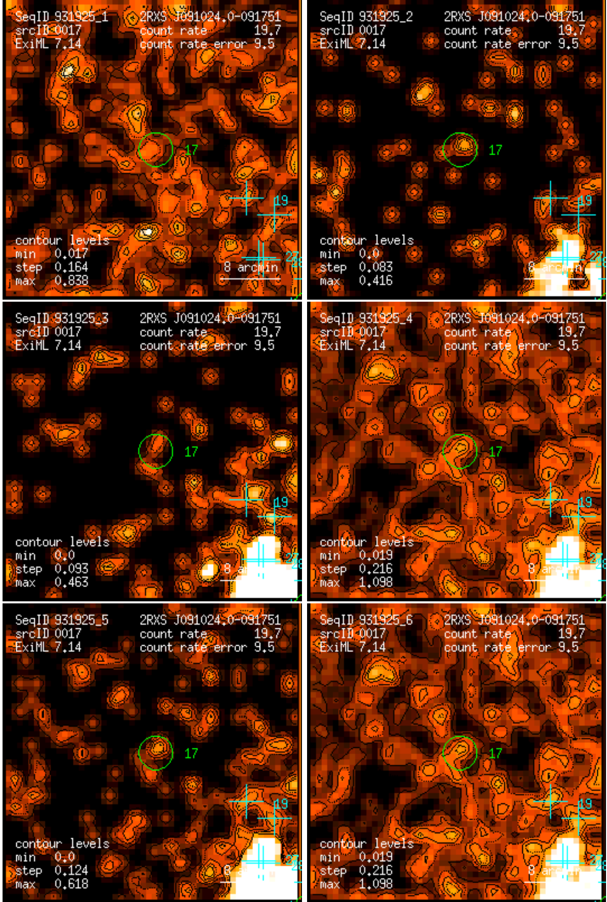
Figure 17: RASS 931925: detection 0017: band rate images, Gaussian filter: (1) PSPC channels 11 – 41, (2) 52 – 90, (3) 91 – 201, (4) 11 – 235, (5) 52 – 201, (6) 11 – 201. Broad band rates in counts/ks. Band rate contour levels in counts/ks/arcmin 2 .
