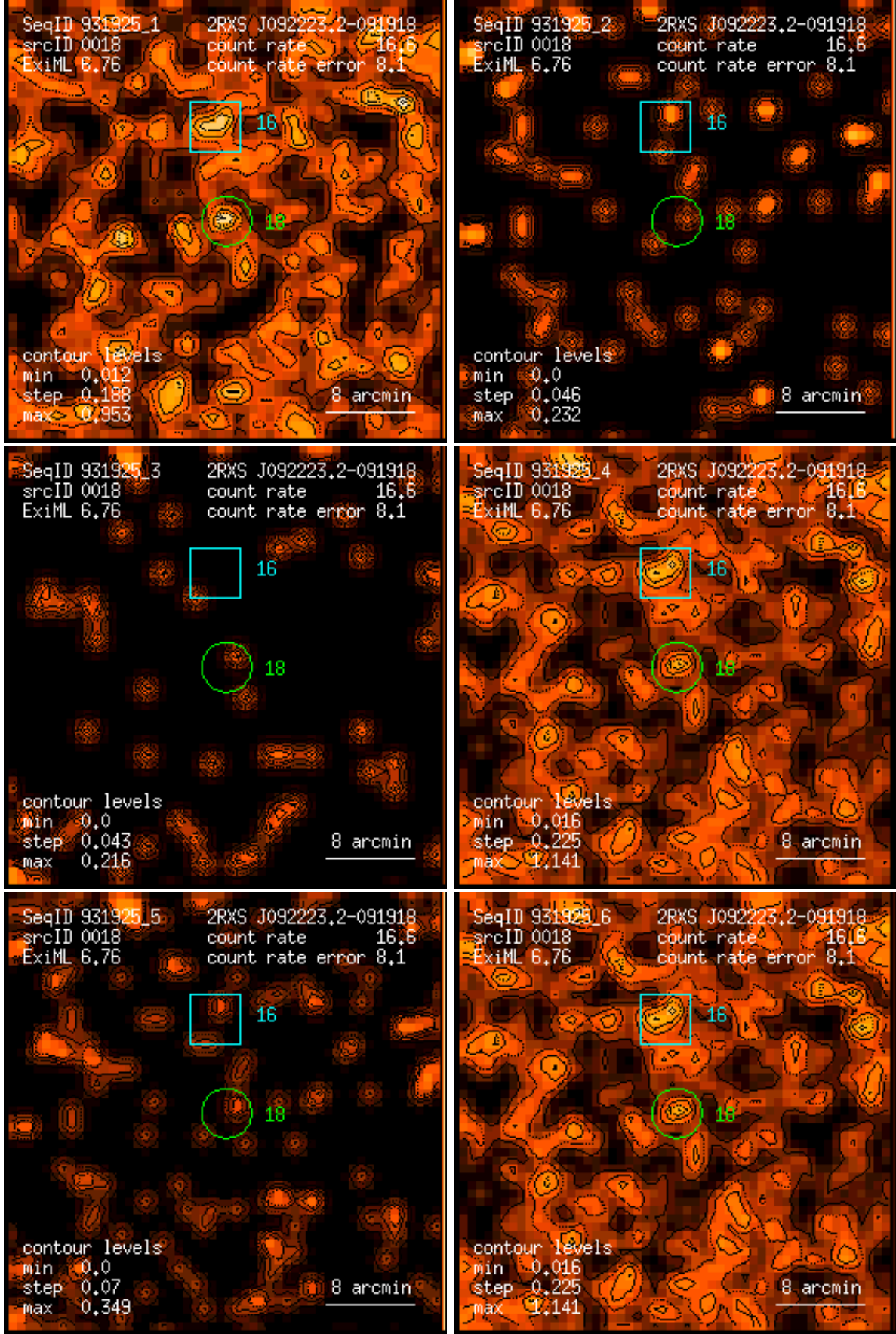
Figure 18: RASS 931925: detection 0018: band rate images, Gaussian filter: (1) PSPC channels 11 – 41, (2) 52 – 90, (3) 91 – 201, (4) 11 – 235, (5) 52 – 201, (6) 11 – 201. Broad band rates in counts/ks. Band rate contour levels in counts/ks/arcmin 2 .
