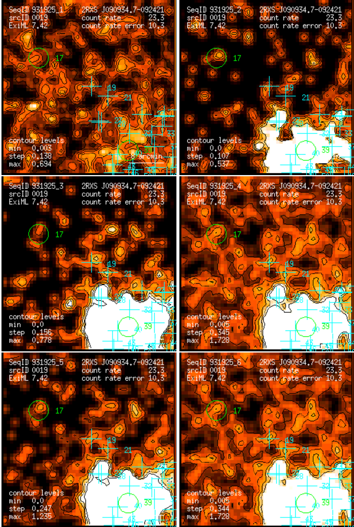
Figure 19: RASS 931925: detection 0019: band rate images, Gaussian filter: (1) PSPC channels 11 – 41, (2) 52 – 90, (3) 91 – 201, (4) 11 – 235, (5) 52 – 201, (6) 11 – 201. Broad band rates in counts/ks. Band rate contour levels in counts/ks/arcmin 2 .
