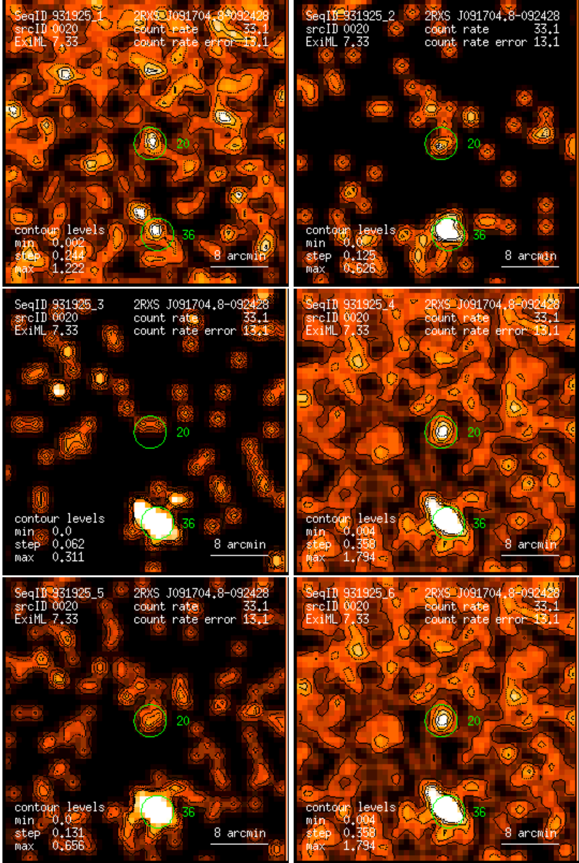
Figure 20: RASS 931925: detection 0020: band rate images, Gaussian filter: (1) PSPC channels 11 – 41, (2) 52 – 90, (3) 91 – 201, (4) 11 – 235, (5) 52 – 201, (6) 11 – 201. Broad band rates in counts/ks. Band rate contour levels in counts/ks/arcmin 2 .
