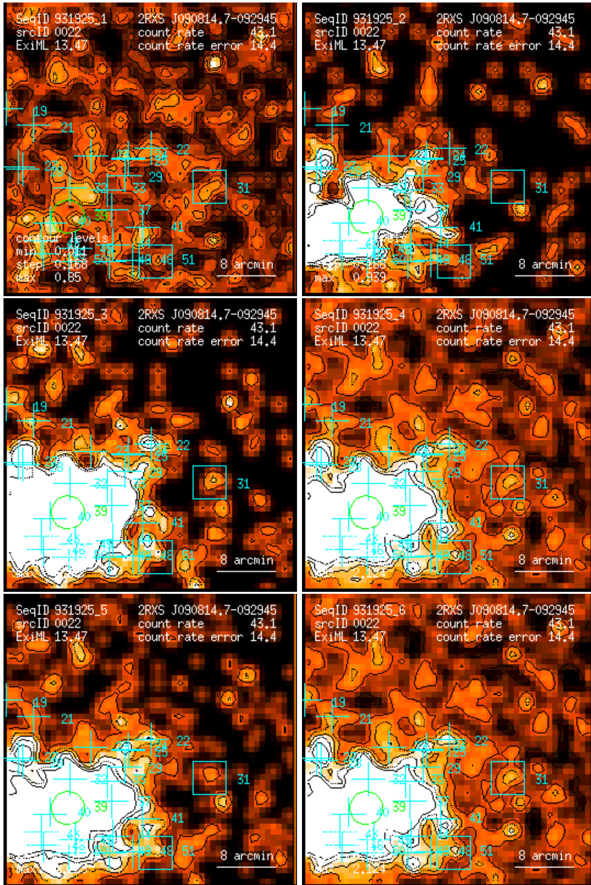
Figure 22: RASS 931925: detection 0022: band rate images, Gaussian filter: (1) PSPC channels 11 – 41, (2) 52 – 90, (3) 91 – 201, (4) 11 – 235, (5) 52 – 201, (6) 11 – 201. Broad band rates in counts/ks. Band rate contour levels in counts/ks/arcmin 2 .
