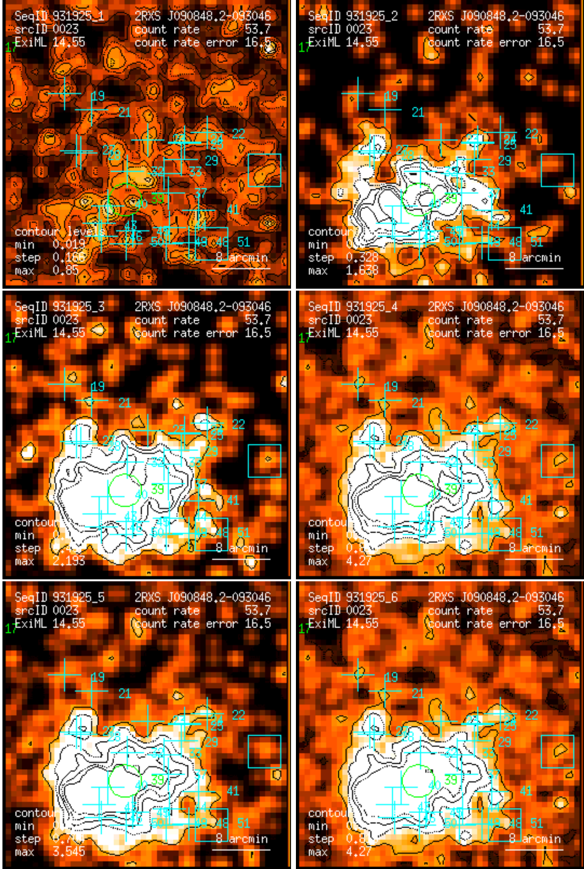
Figure 23: RASS 931925: detection 0023: band rate images, Gaussian filter: (1) PSPC channels 11 – 41, (2) 52 – 90, (3) 91 – 201, (4) 11 – 235, (5) 52 – 201, (6) 11 – 201. Broad band rates in counts/ks. Band rate contour levels in counts/ks/arcmin 2 .
