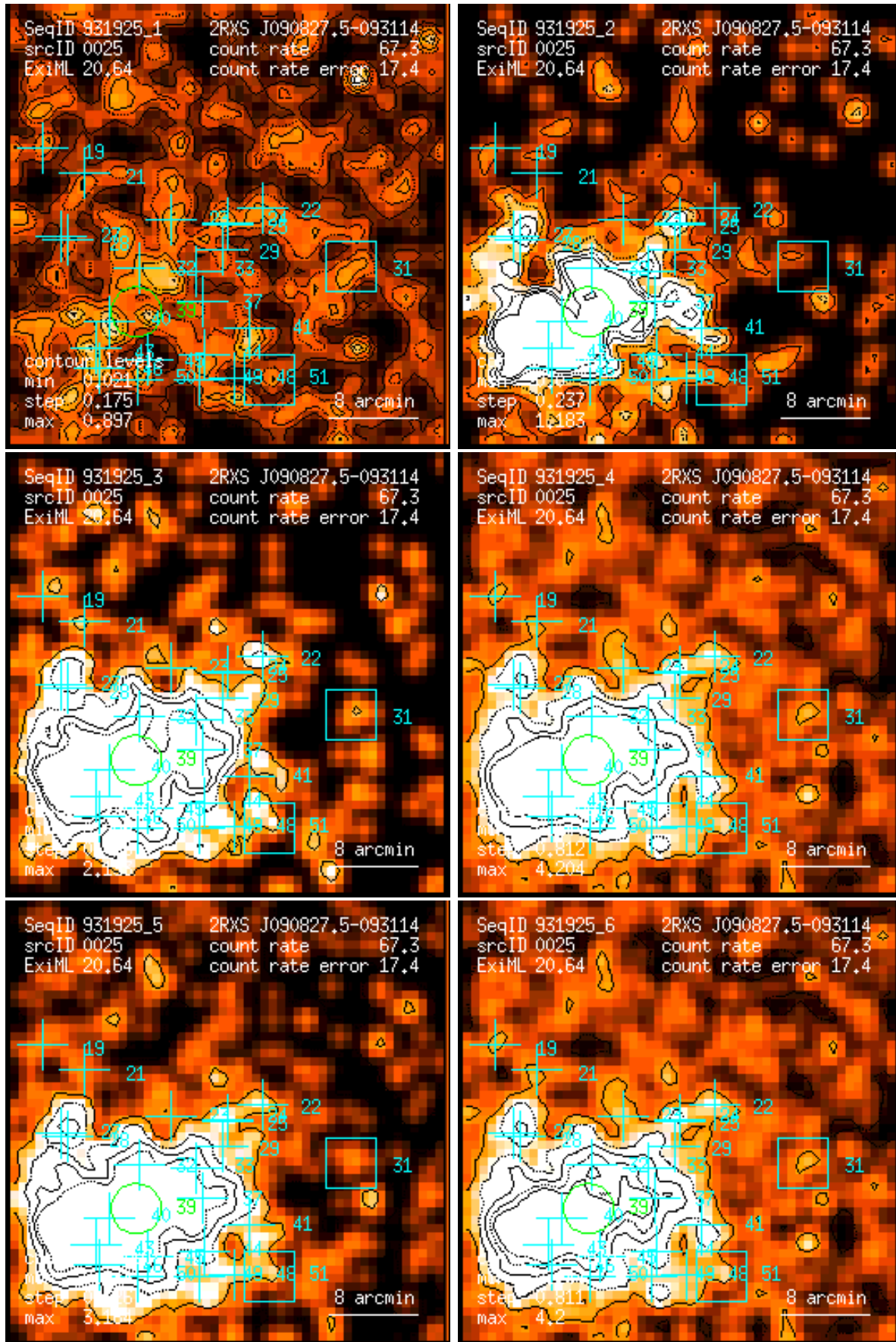
Figure 25: RASS 931925: detection 0025: band rate images, Gaussian filter: (1) PSPC channels 11 – 41, (2) 52 – 90, (3) 91 – 201, (4) 11 – 235, (5) 52 – 201, (6) 11 – 201. Broad band rates in counts/ks. Band rate contour levels in counts/ks/arcmin 2 .
