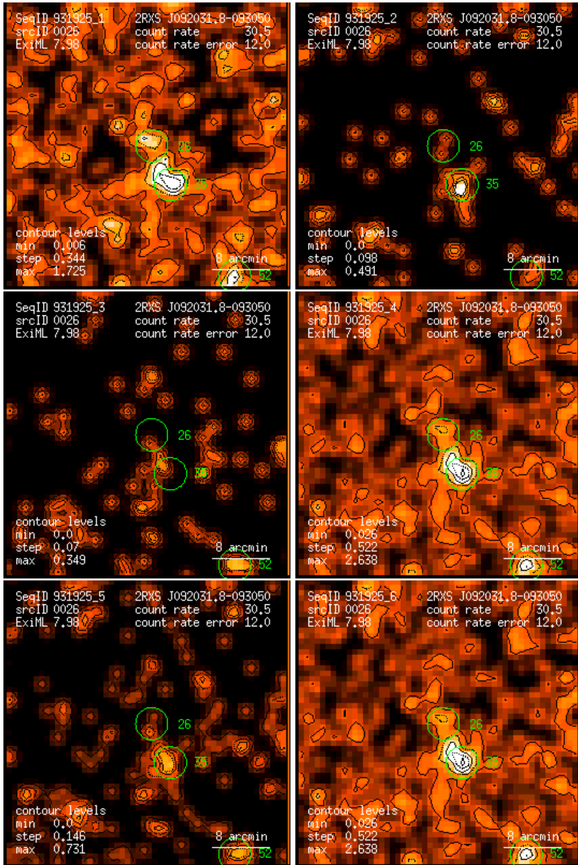
Figure 26: RASS 931925: detection 0026: band rate images, Gaussian filter: (1) PSPC channels 11 – 41, (2) 52 – 90, (3) 91 – 201, (4) 11 – 235, (5) 52 – 201, (6) 11 – 201. Broad band rates in counts/ks. Band rate contour levels in counts/ks/arcmin 2 .
